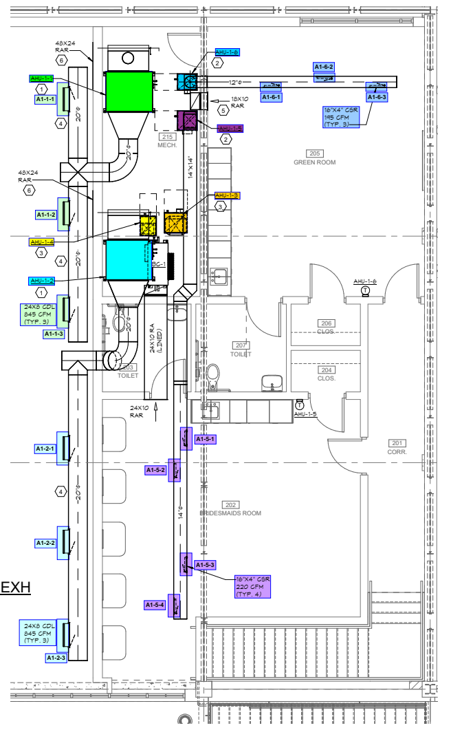
1 SECOND FLOOR SOUTH - ENLARGED MECHANICAL PLAN M2.4
