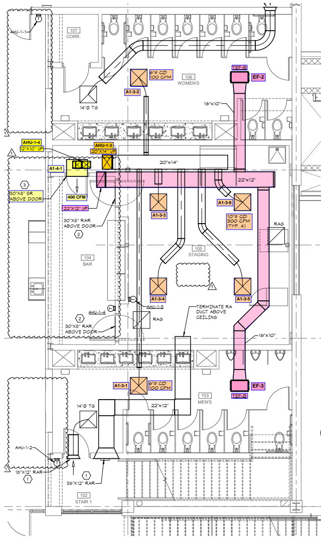
1 FIRST FLOOR SOUTH - ENLARGED MECHANICAL PLAN M2.2
