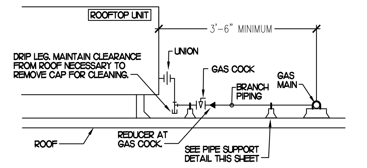
3 GAS PIPING AT RTU NO SCALE
