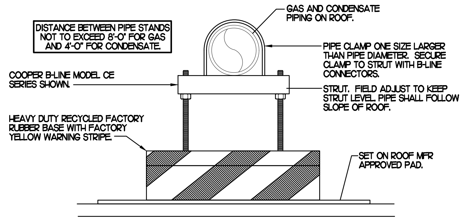
4 PIPING SUPPORT NO SCALE
