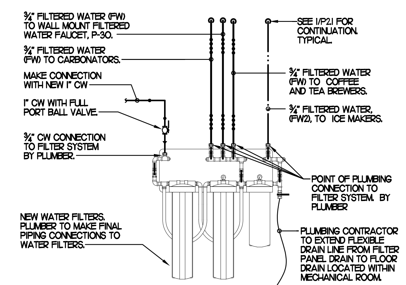
9 WATER FILTER RISER PIPING SCALE: NONE
