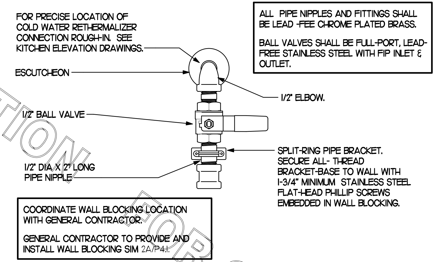
1 RETHERMALIZER WATER SUPPLY VALVE SCALE: NONE
