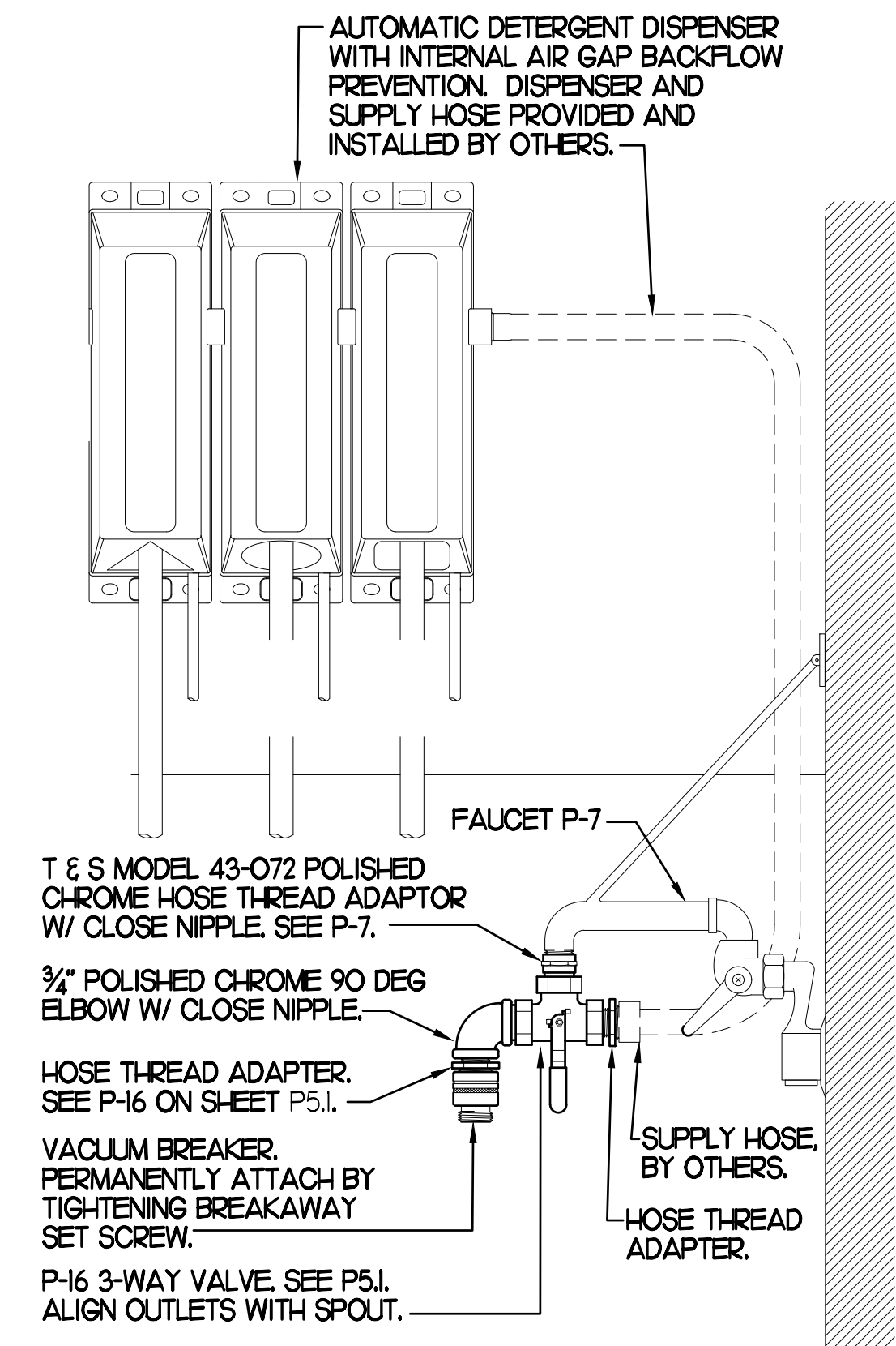
4 3-WAY VALVE AT MOP SINK SCALE: NONE
