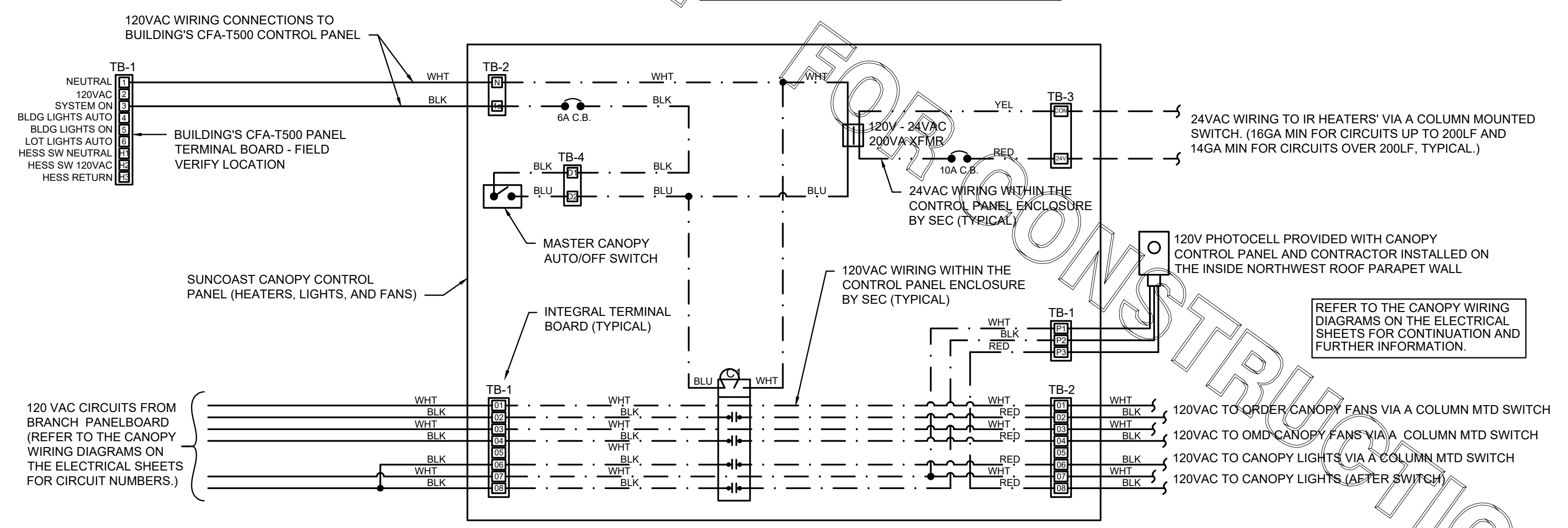
1 SUNCOAST PANEL WIRING DIAGRAM - INFRARED HEATERS, COOLING FANS NO SCALE
