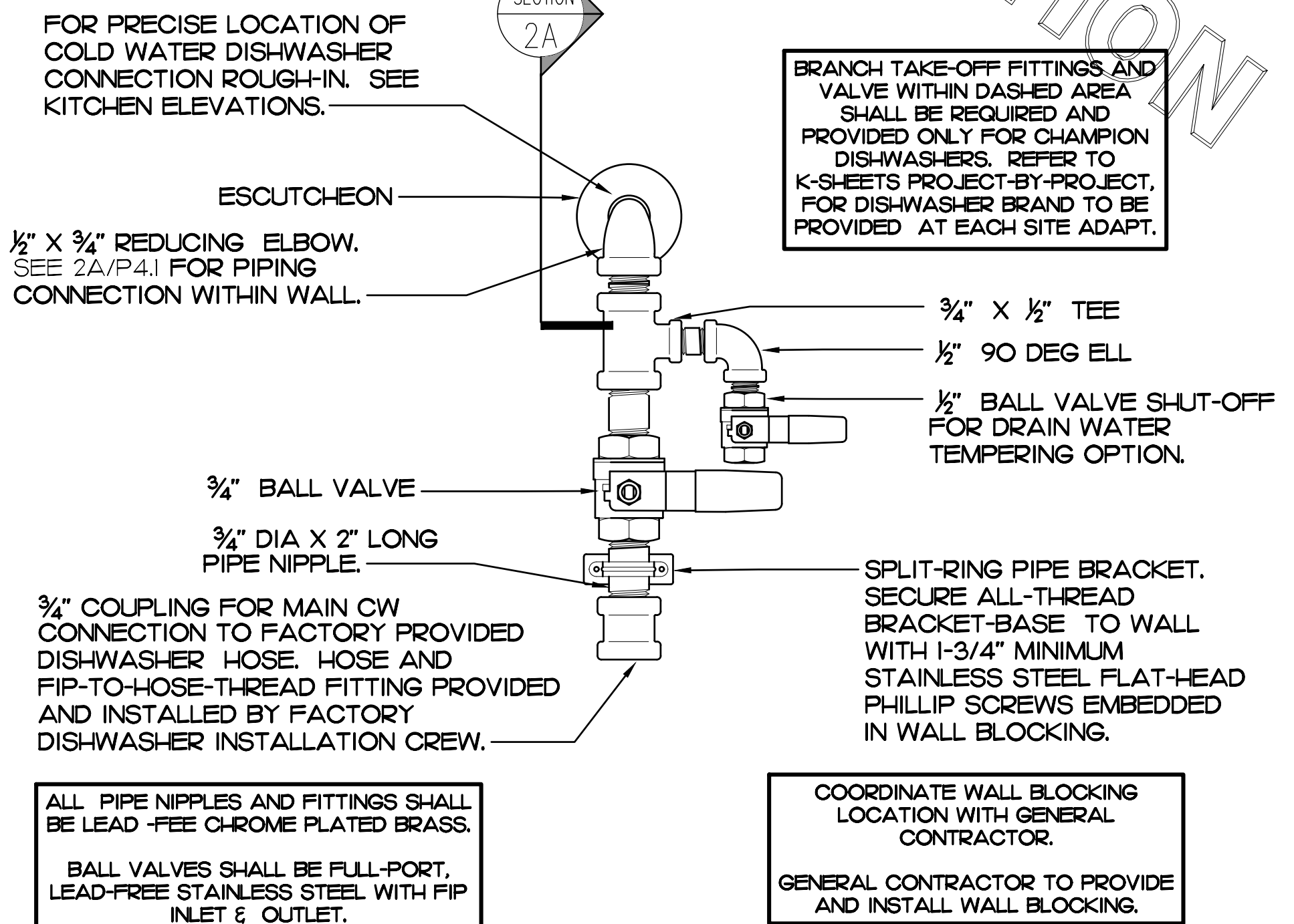
2 DISHWASHER WATER SUPPLY VALVE ASSEMBLY SCALE: NONE
