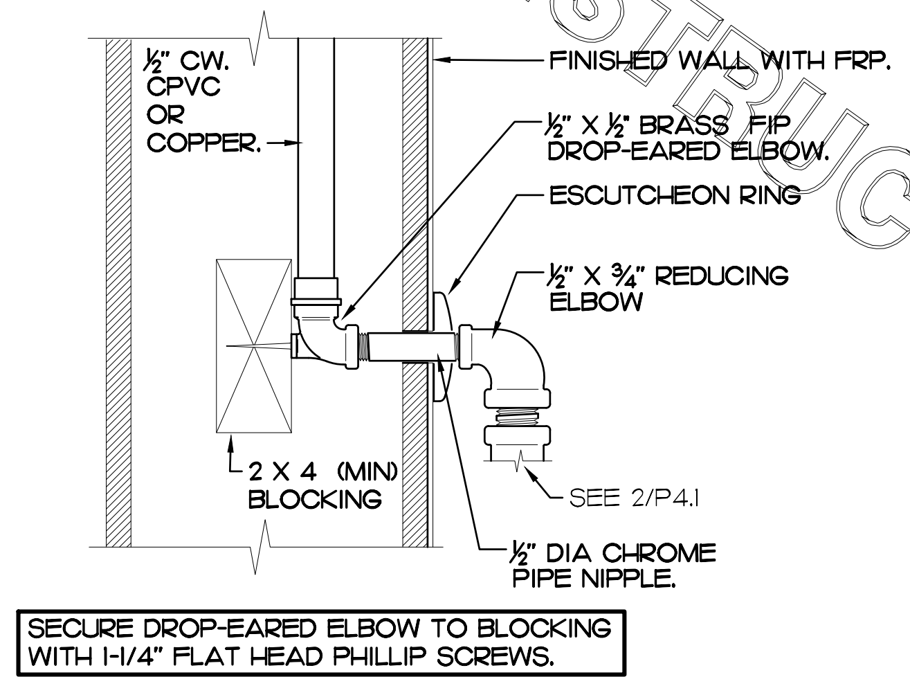
2A SECTION AT PIPING WITHIN WALL SCALE: NONE
