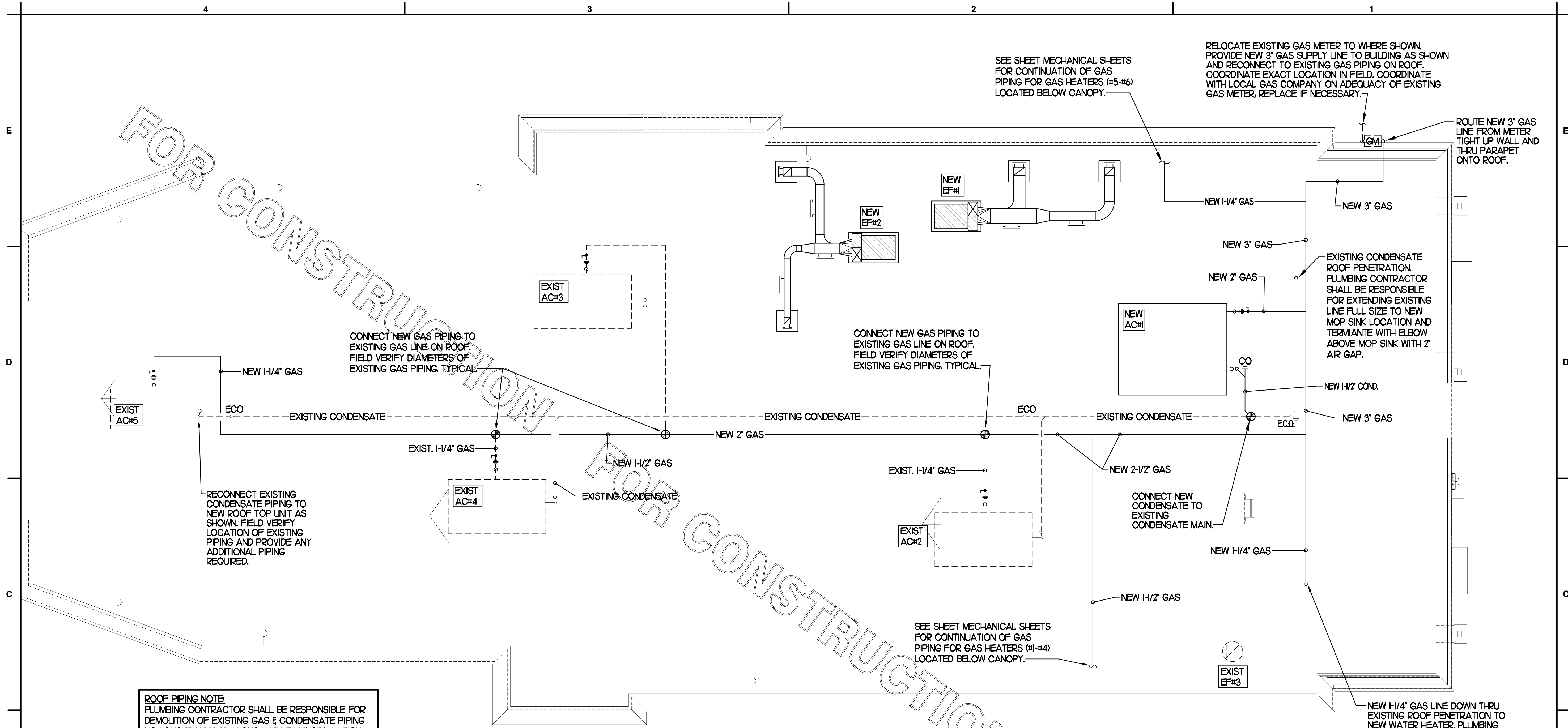
1 PLUMBING ROOF PLAN SCALE: 1/4"=1'-0"
