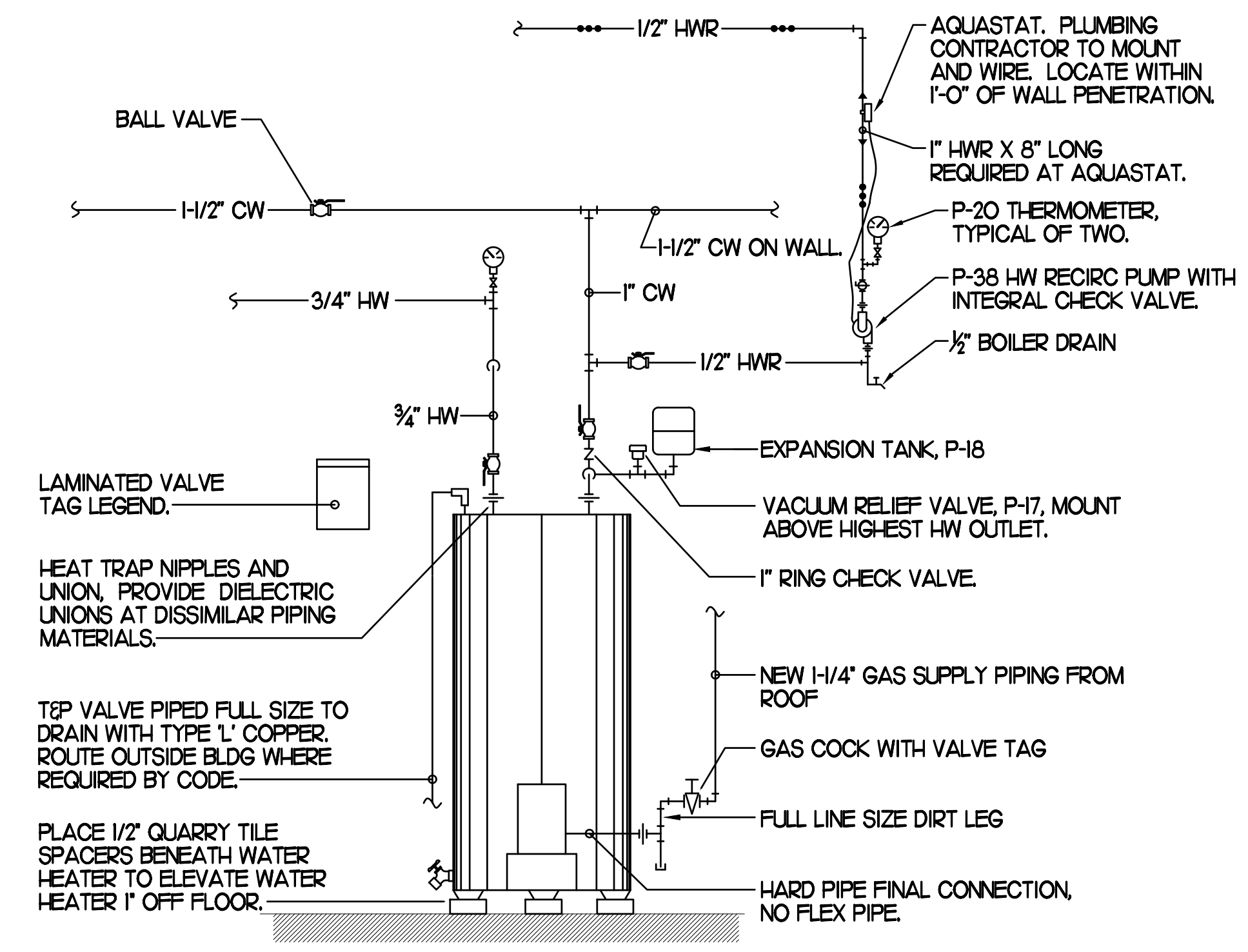
5 WATER HEATER PIPING SCALE: NONE
