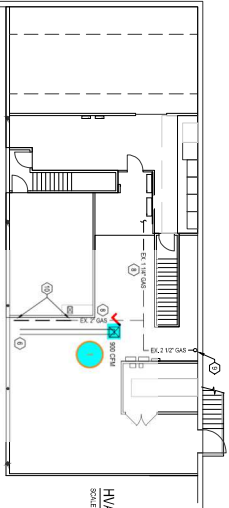
HVAC MEZZANINE FLOOR PLAN SCALE 1:200
