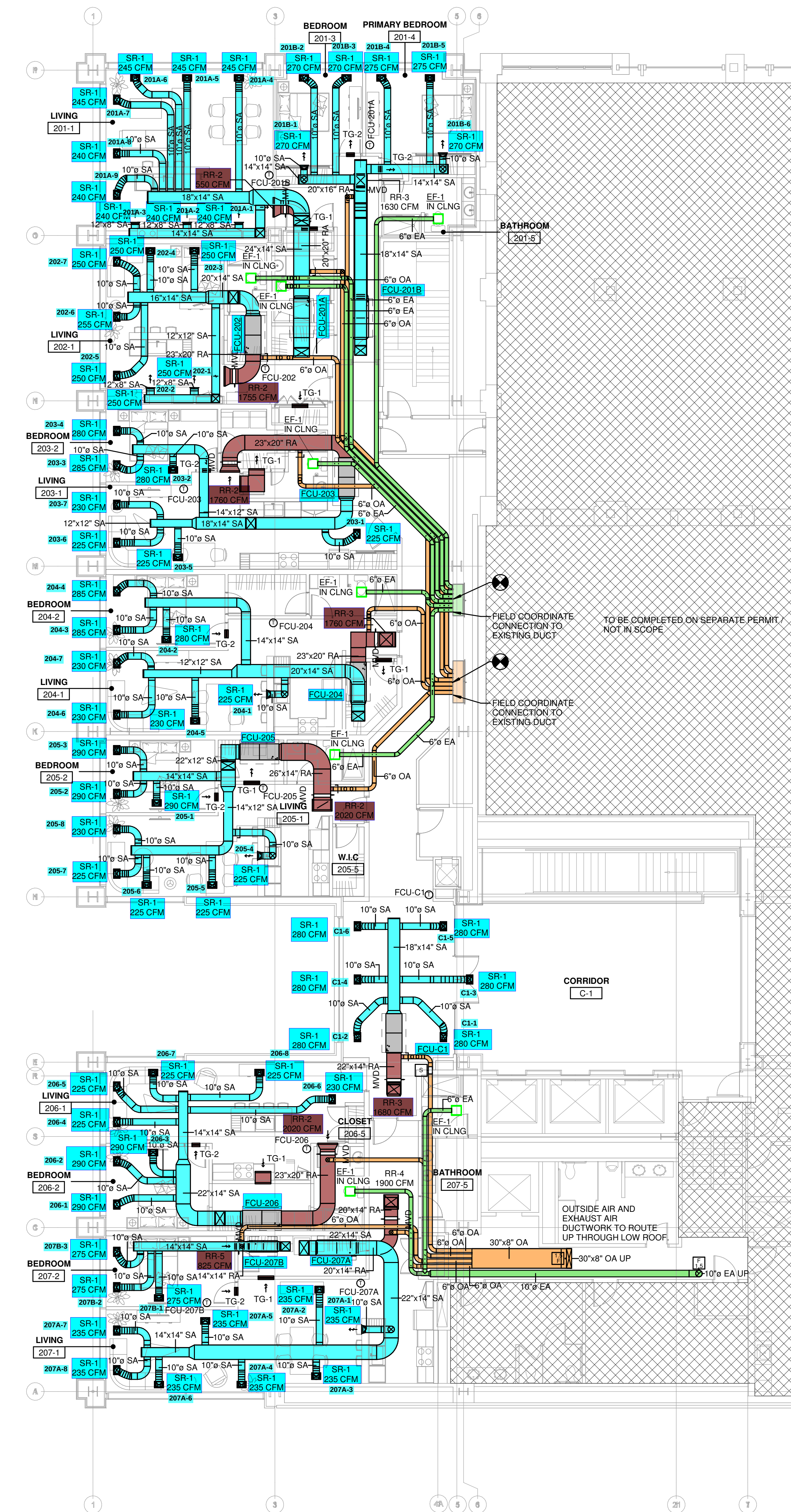
① MECHANICAL PLAN - LEVEL 2 1/8" = 1'-0"
