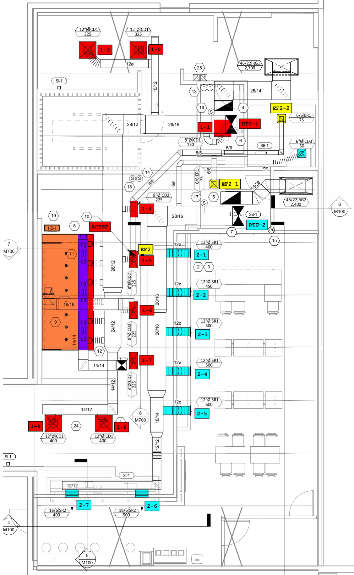
1 HVAC FLOOR PLAN 1/4" = 1'-0"
