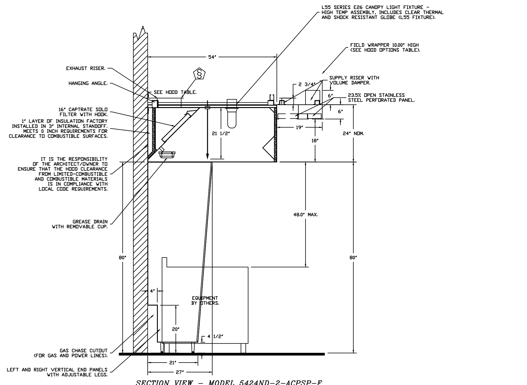
SECTION VIEW - MODEL 5424ND-2-ACPS-P HOOD - #1
