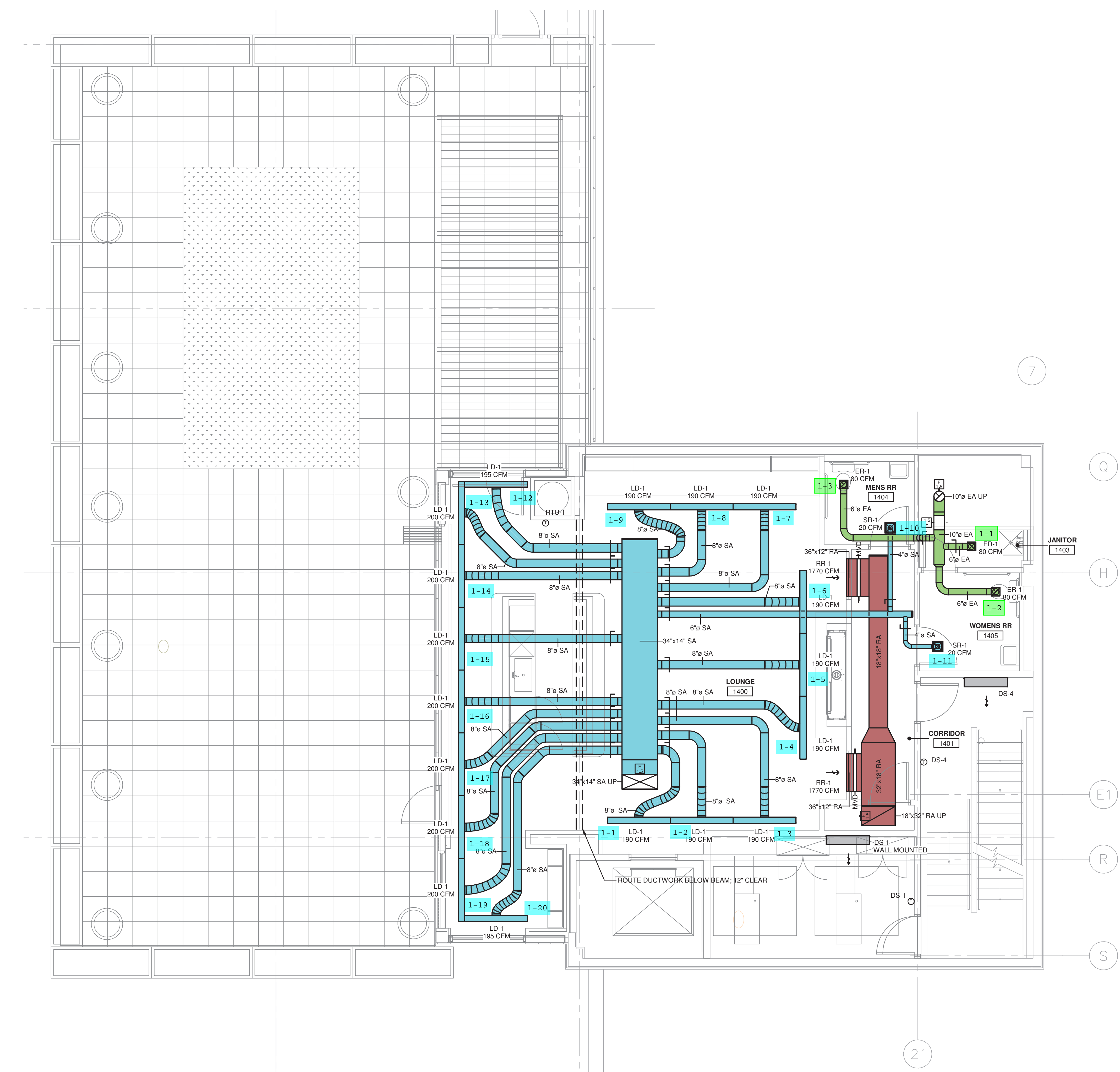
1 MECHANICAL PLAN - LEVEL 14 - LOUNGE 1/4" = 1'-0"
