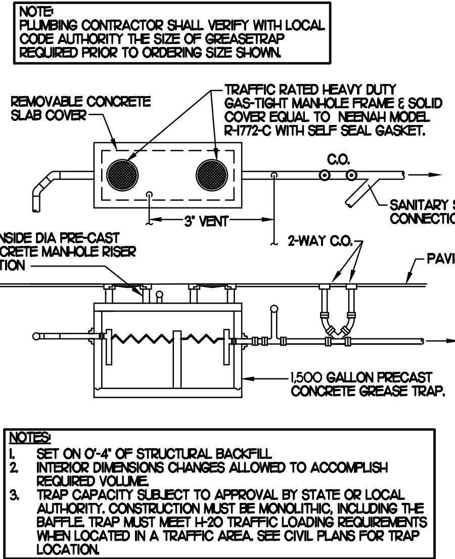
2 GREASE INTERCEPTOR SCALE: NONE
