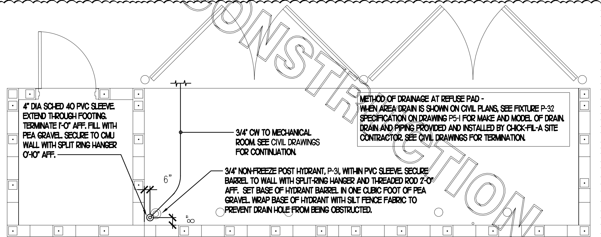
3 REFUSE PAD PLUMBING SCALE: NONE
