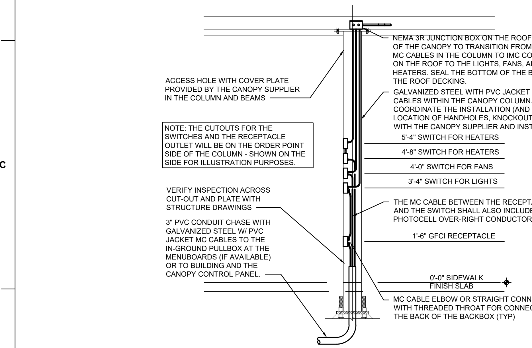
ORDER CANOPY COLUMN SECTION NOT TO SCALE
