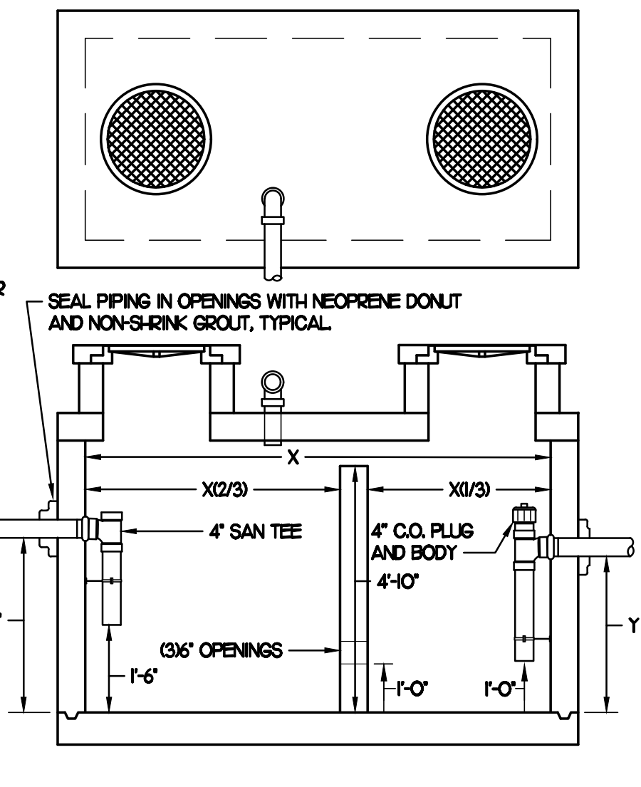
4 SAN. C.O. OUTSIDE BUILDING SCALE: NONE
