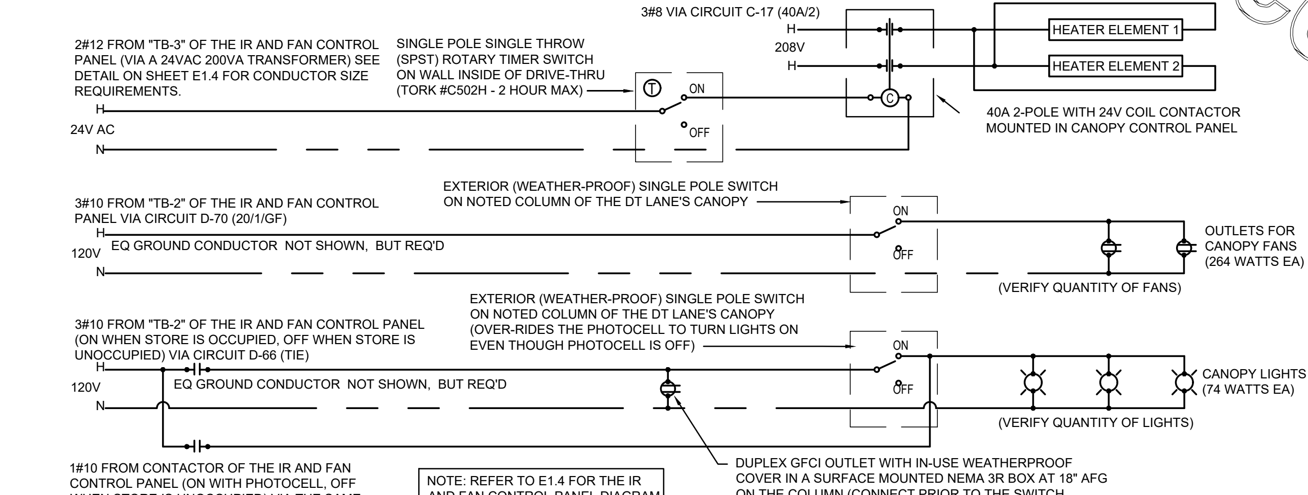
OMD CANOPY POWER WIRING SCHEMATIC NOT TO SCALE
