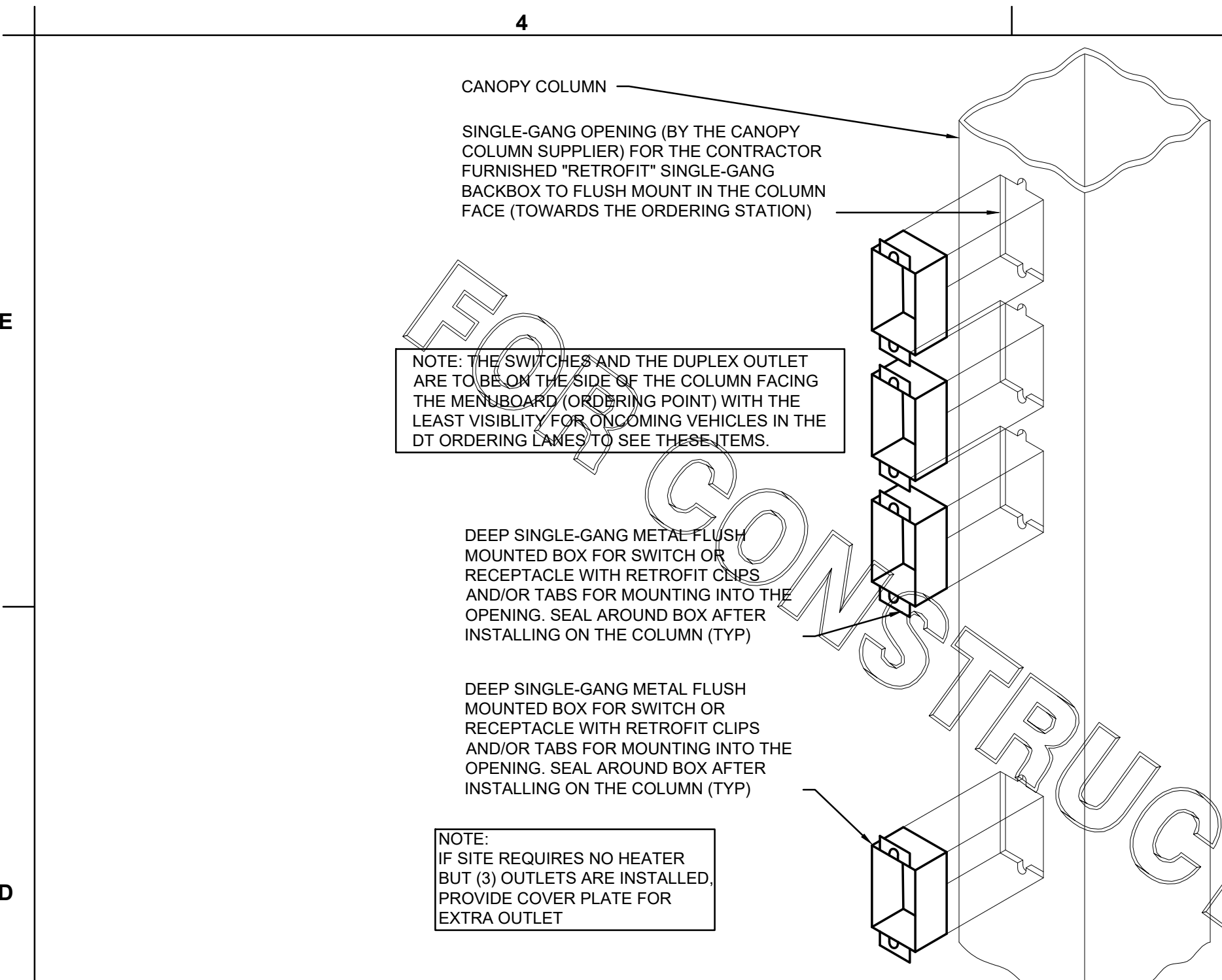
CANOPY COLUMN ISOMETRIC NOT TO SCALE
