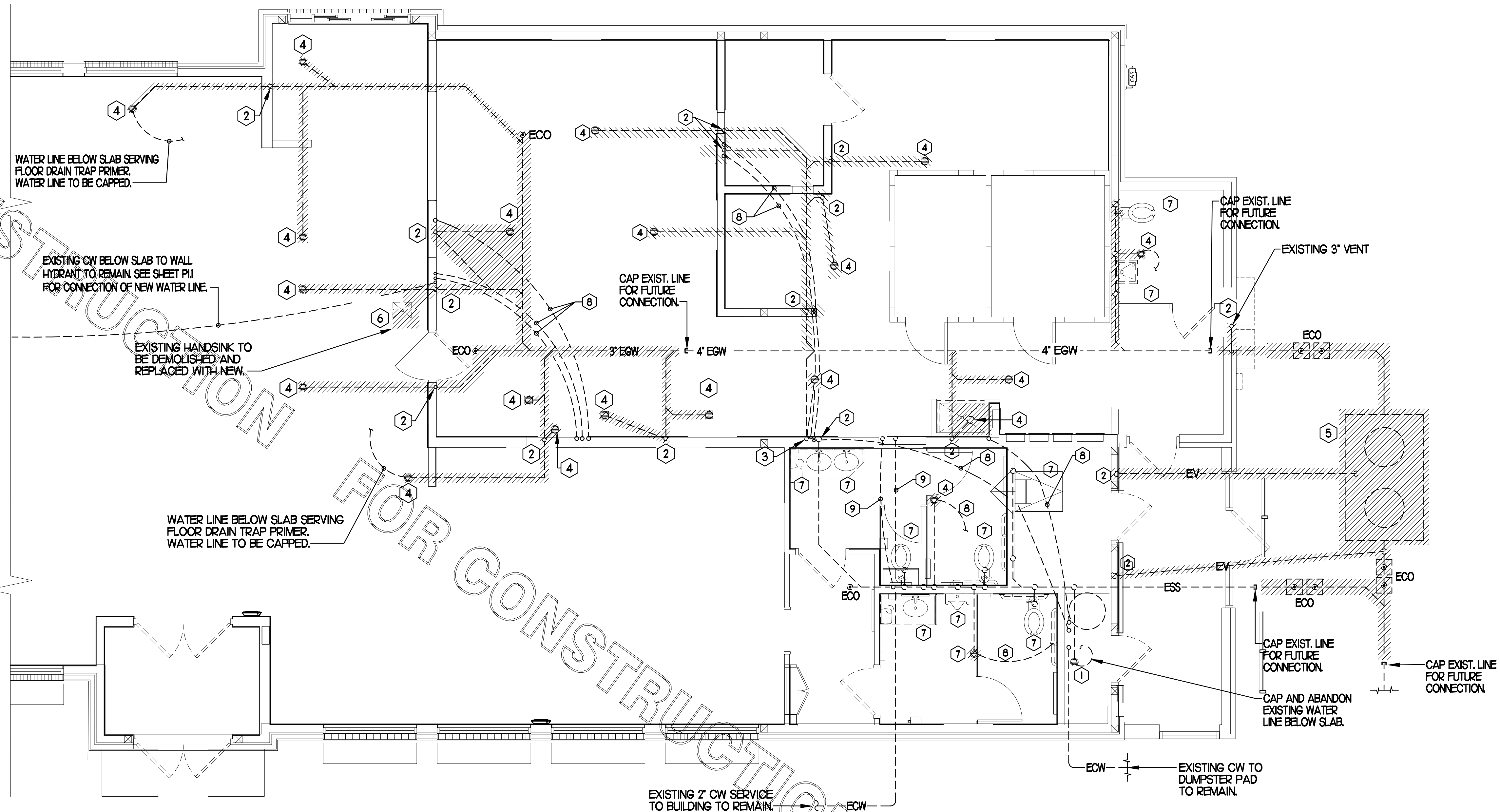
1 BELOW SLAB PLUMBING DEMOLITION PLAN SCALE: 1/4"=1'-0"
