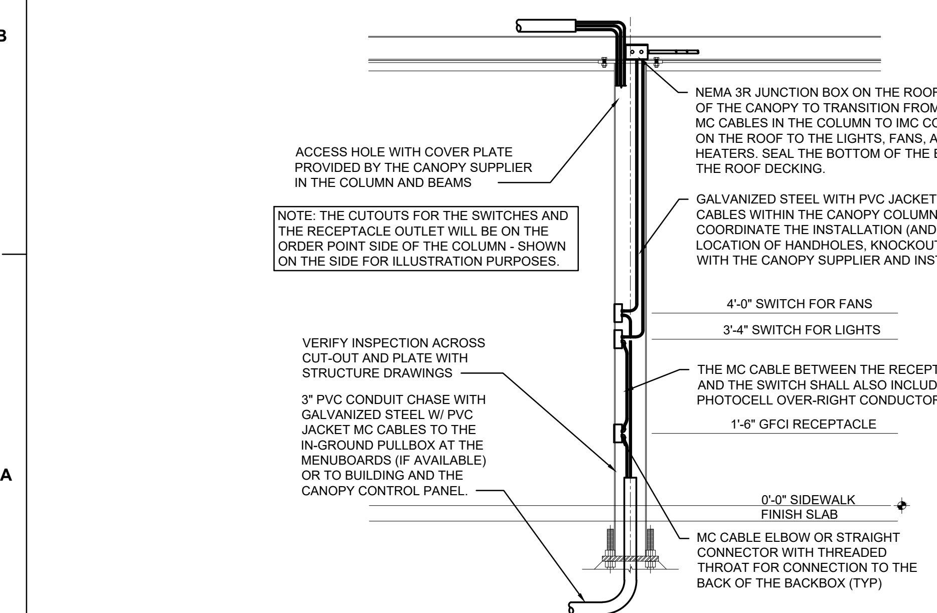
OMD CANOPY COLUMN SECTION NOT TO SCALE
