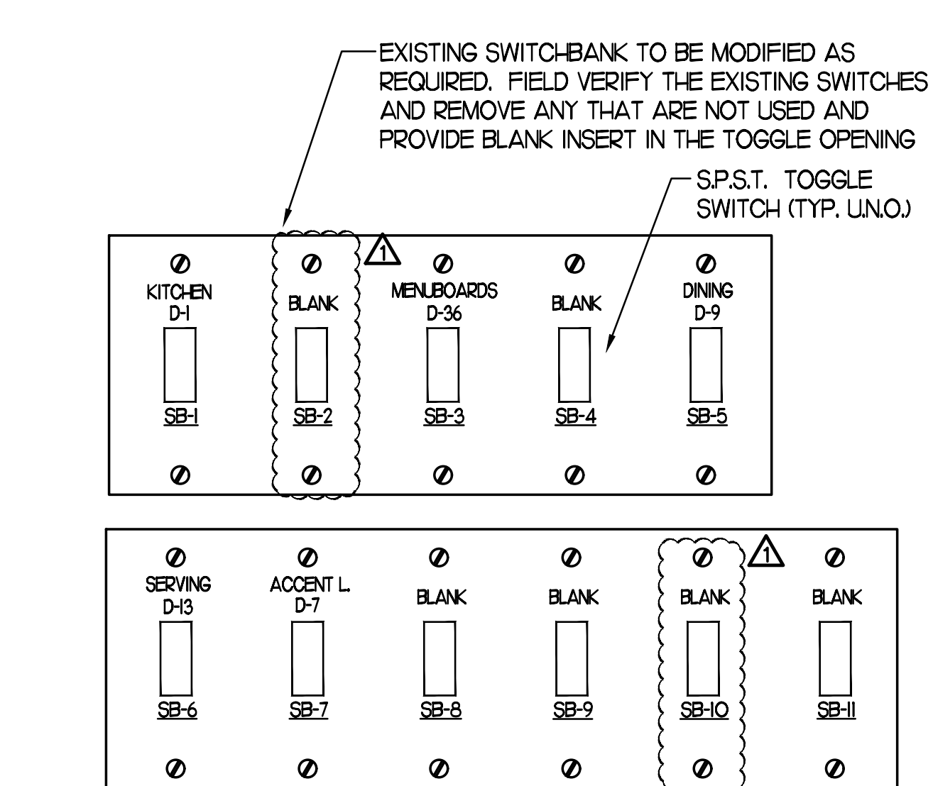
6 RELOCATED SWITCH BANK "SB" DETAIL NO SCALE
