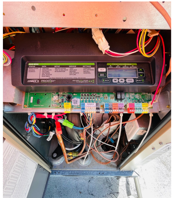
Missing HUM Wiring
