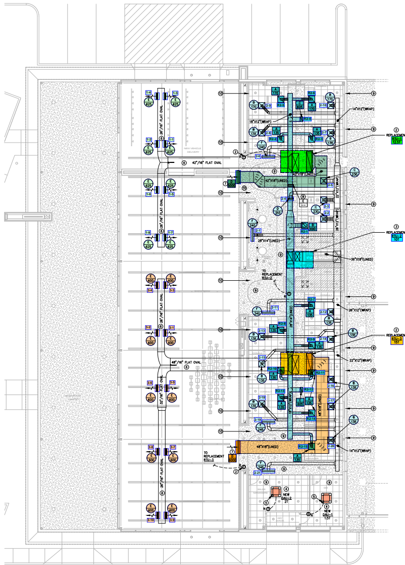
1 SHOWROOM FLOOR PLAN – MECHANICAL SCALE: 1/8" = 1'-0"
