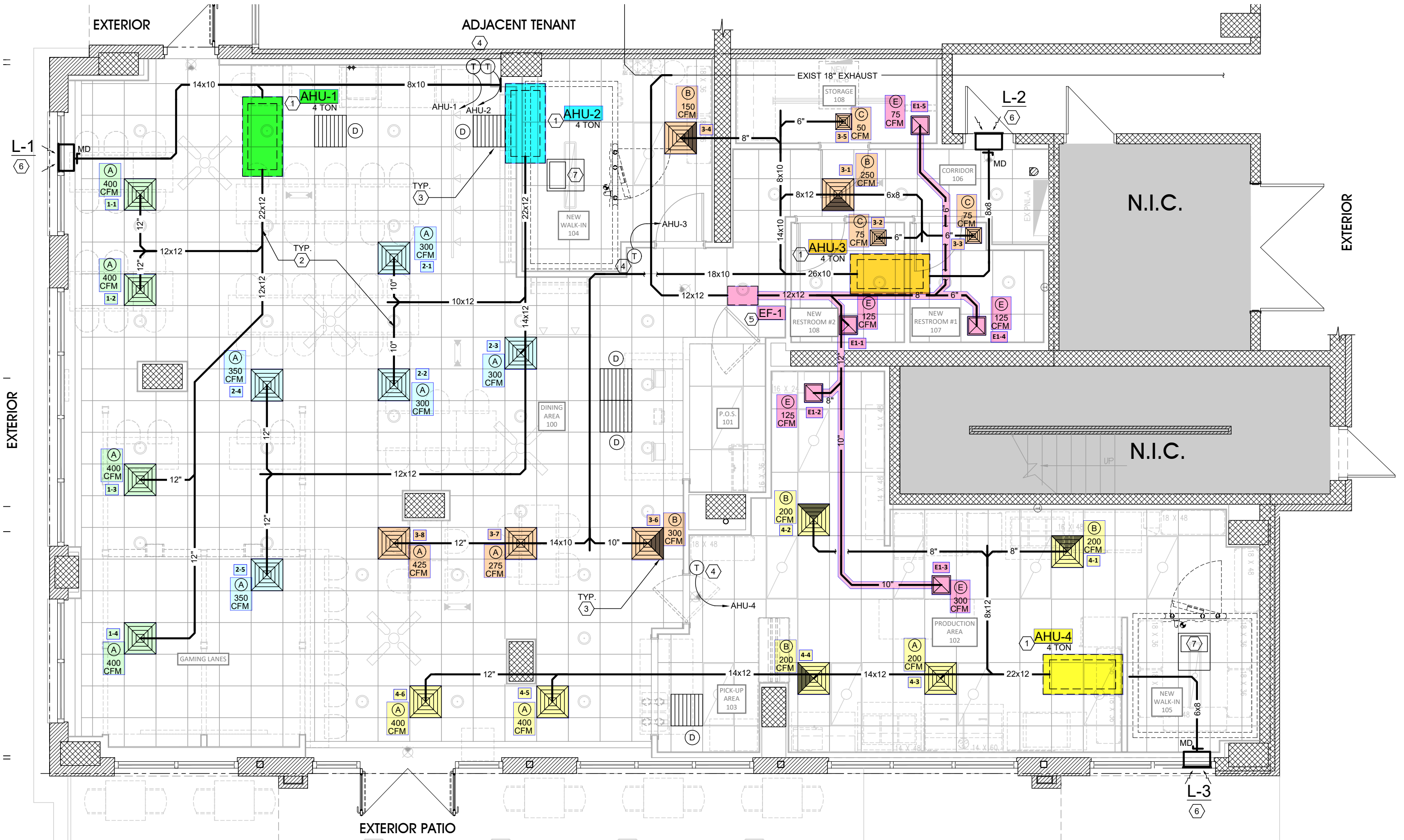
Mechanical HVAC Plan
