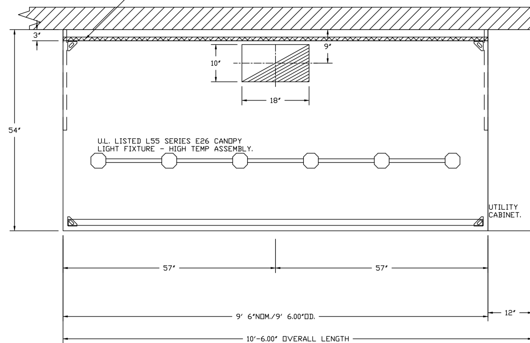
PLAN VIEW - HOOD #1 9' 6.00" LONG 5424ND-2
