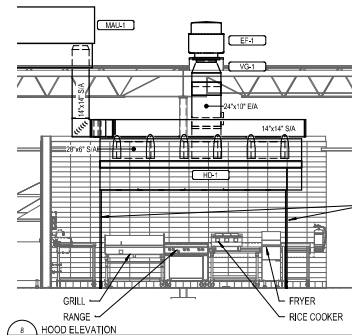
8 HOOD ELEVATION M700 NOT TO SCALE
