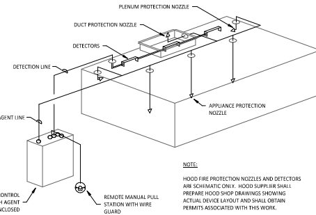
4 FIRE SUPPRESSION SYSTEM SCHEMATIC M700 NOT TO SCALE
