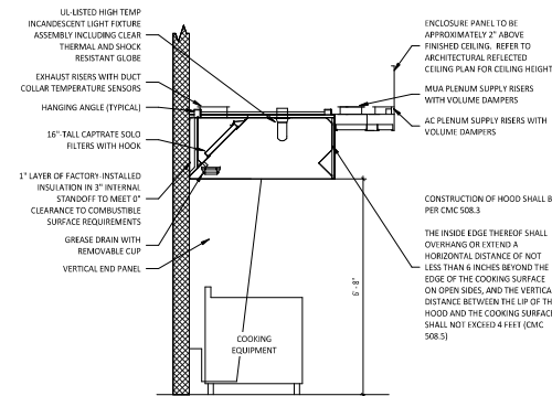
2 HOOD SECTION VIEW M700 NOT TO SCALE
