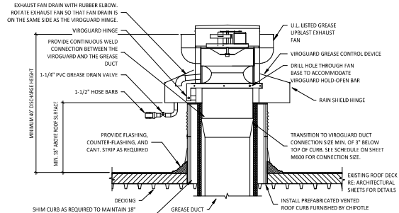
5 GREASE EXHAUST FAN M700 NOT TO SCALE
