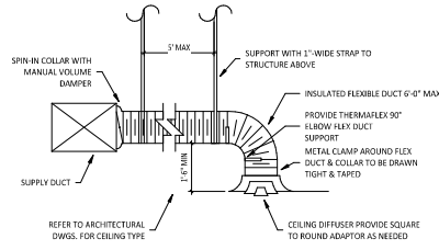
1 DIFFUSER CONNECTION M700 NOT TO SCALE
