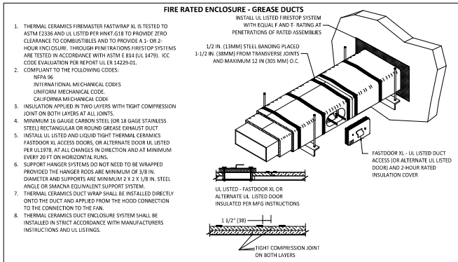
3 FIREMASTER DUCT WRAP - UL-HNK-G16 M700 NOT TO SCALE
