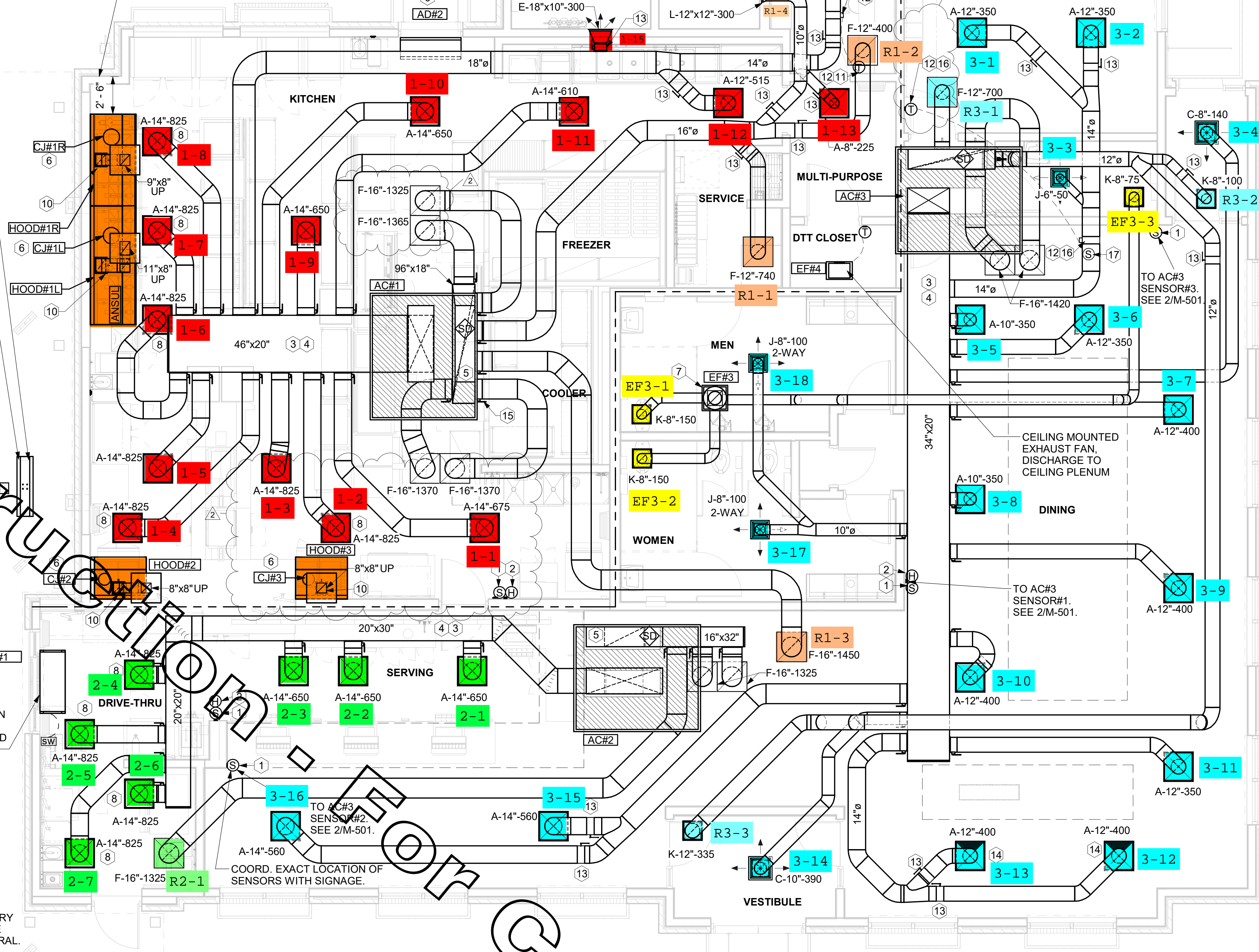
1 MECHANICAL FLOOR PLAN 1/4" = 1'-0"
