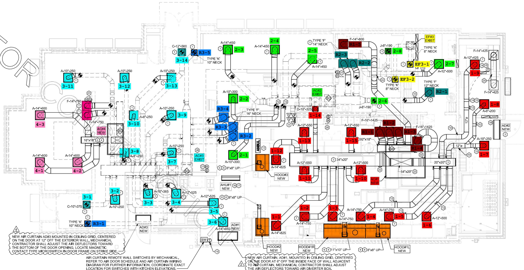
1 MECHANICAL FLOOR PLAN 1/4" = 1'-0"
