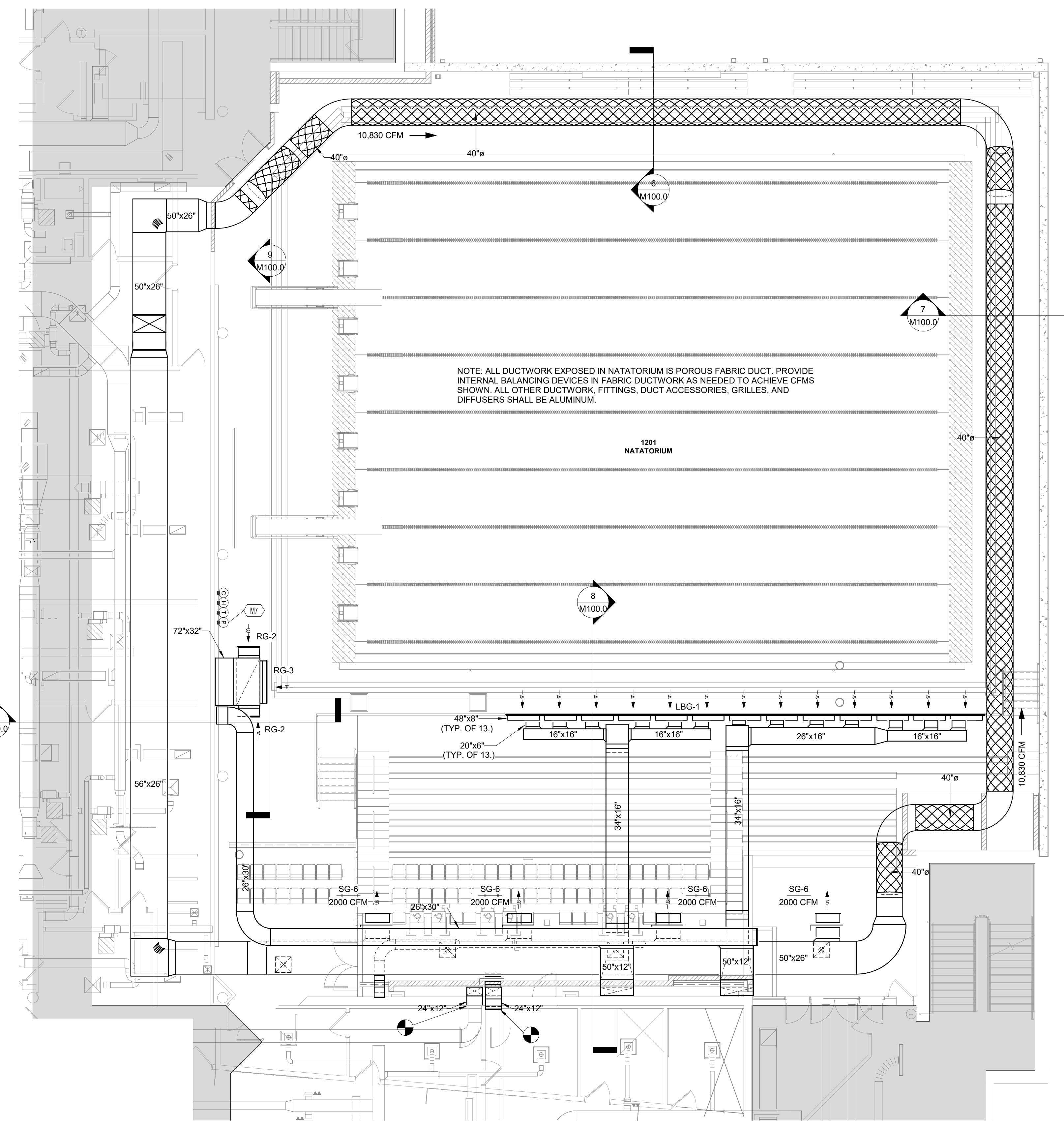
1 NATATORIUM DUCTWORK PLAN M100.0 1/8" = 1'-0"
