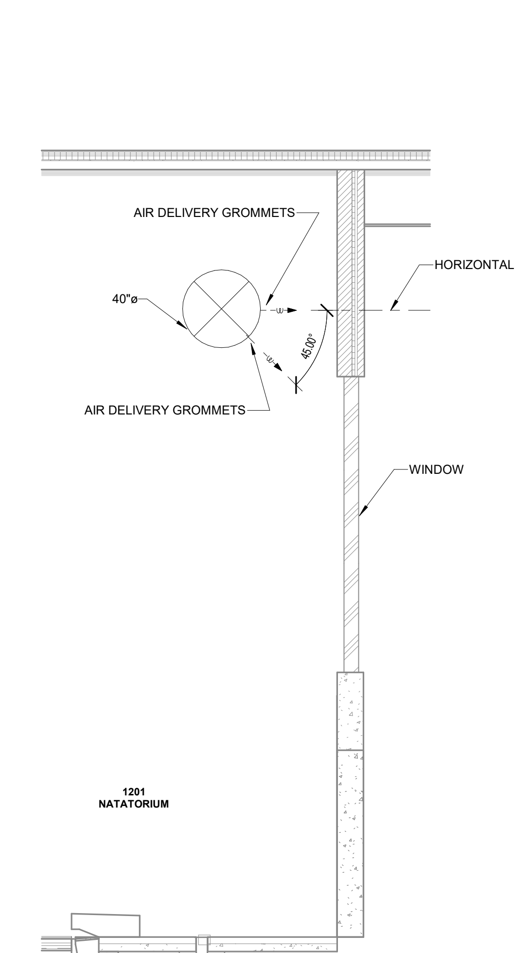
7 EAST WALL SECTION VIEW M100.0 1/4" = 1'-0"
