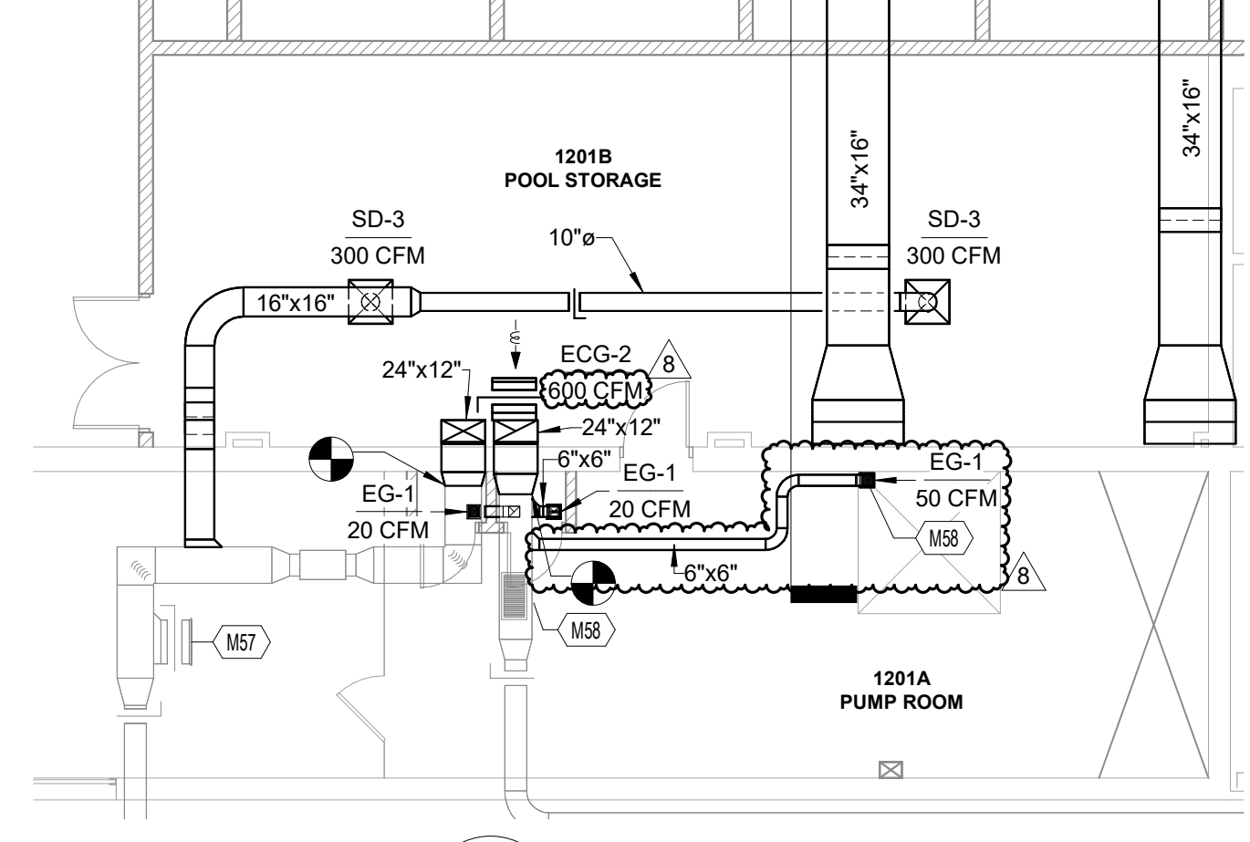
2 POOL STORAGE PLAN M100.0 1/8" = 1'-0"
