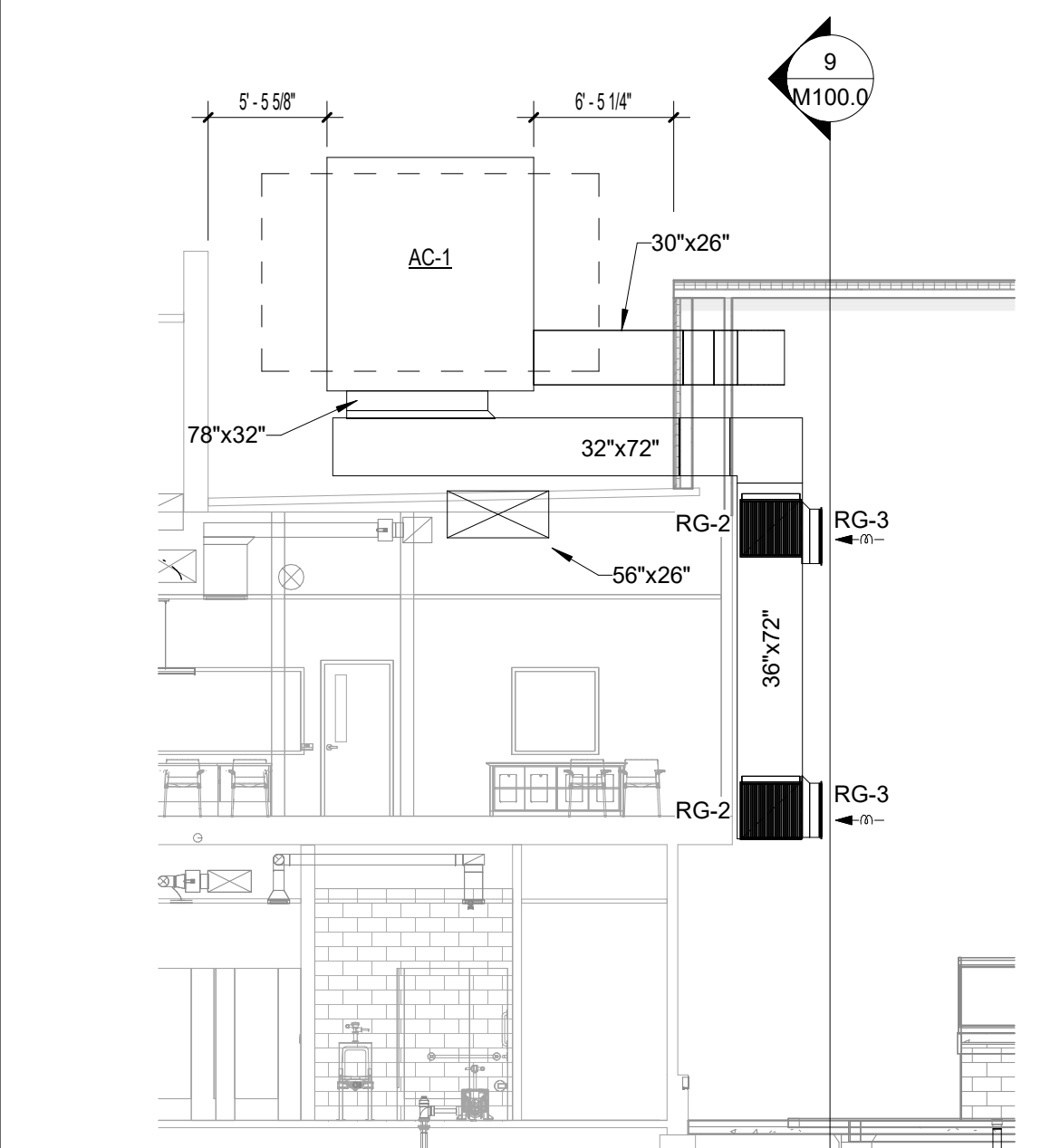
3 POOL RETURN DUCT SECTION VIEW M100.0 1/8" = 1'-0"
