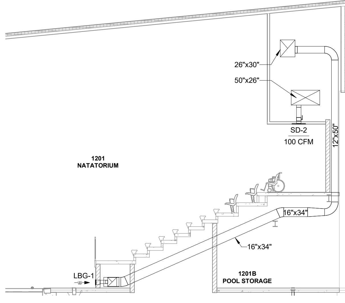
8 LOW EXHAUST DUCT SECTION VIEW M100.0 1/8" = 1'-0"
