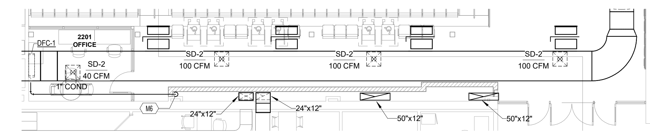
5 UPPER LEVEL DUCTWORK PLAN AREA C (NATATORIUM) M100.0 1/8" = 1'-0"
