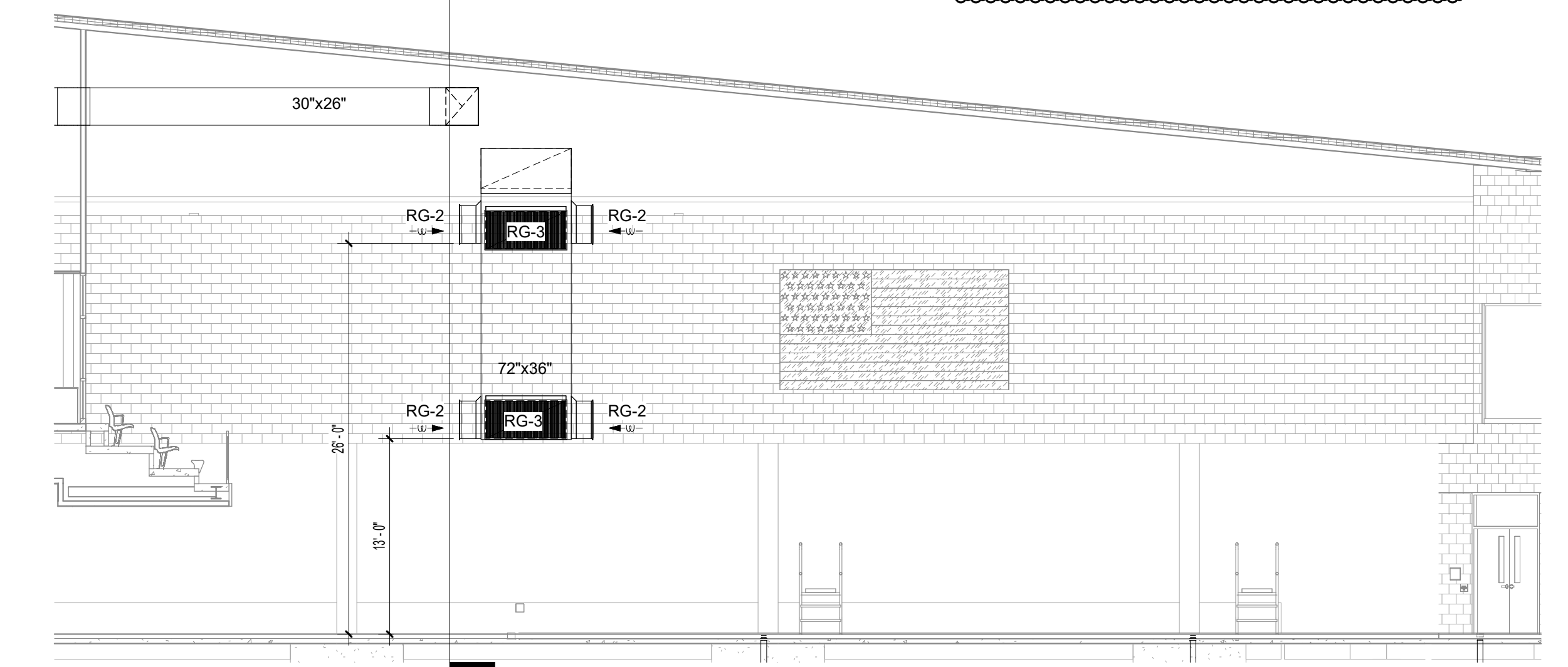
9 POOL RETURN & EXHAUST DUCT SECTION VIEW M100.0 1/8" = 1'-0"
