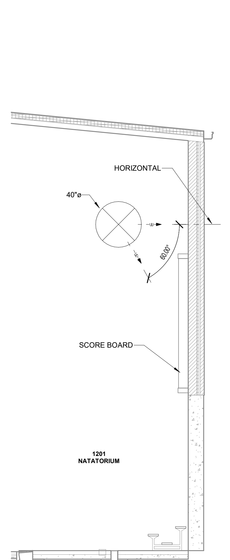
6 NORTH WALL SECTION VIEW M100.0 1/4" = 1'-0"
