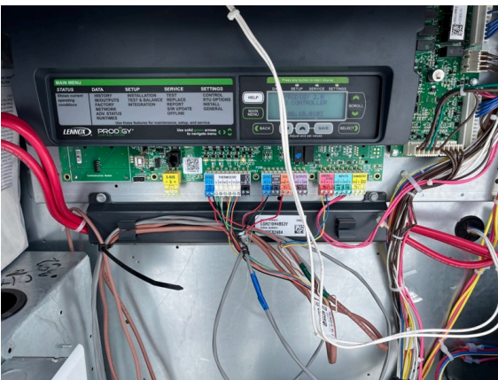
RTU-2 Control wiring
