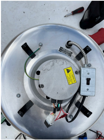
PRV-1 Disconnect installed
