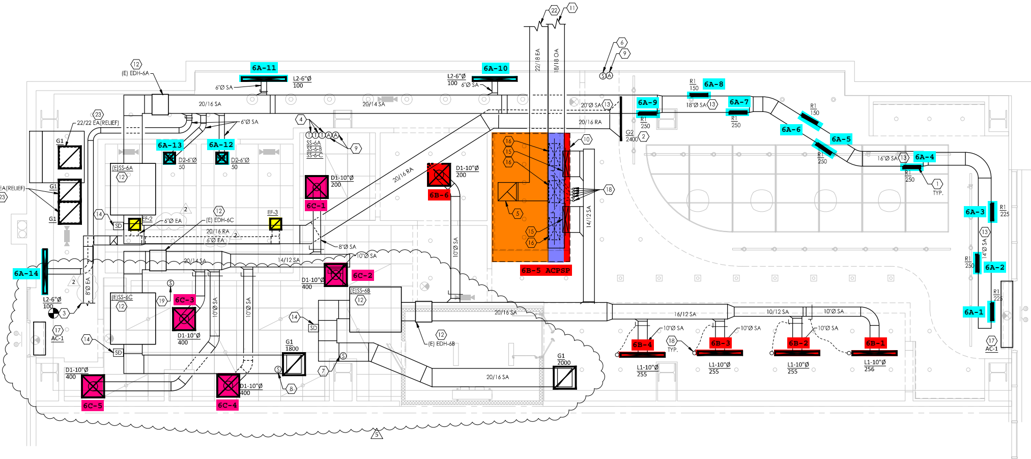
1 MECHANICAL PLAN 1/4" = 1'-0"
