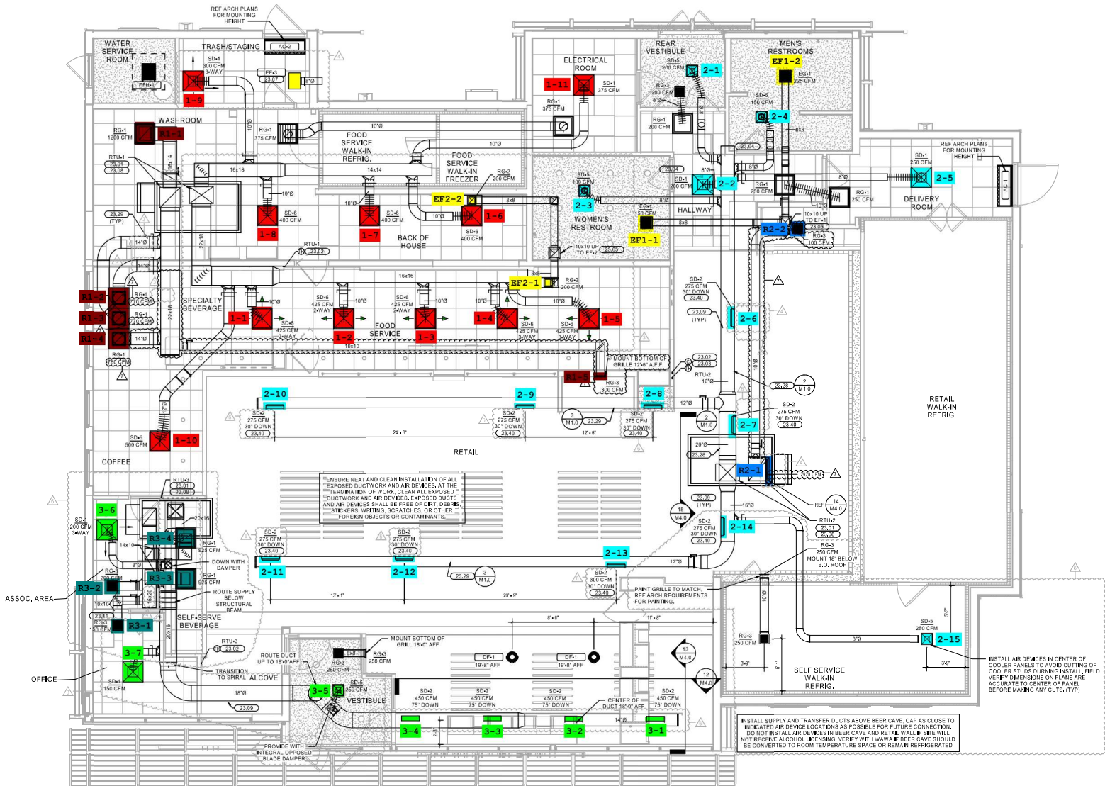
1 HVAC FLOOR PLAN 1/4" = 1'-0"
