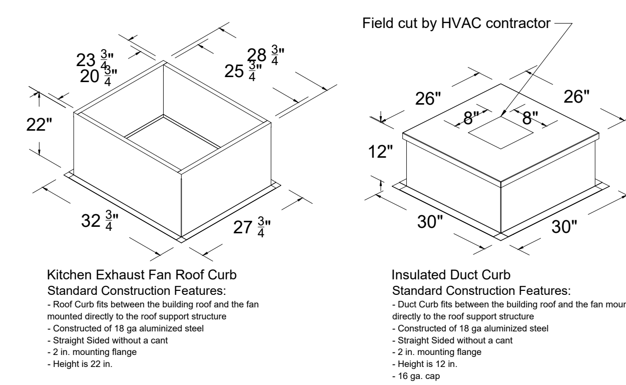
Model: GPI For Model: XRED-090-VG Curb & Damper Tray
