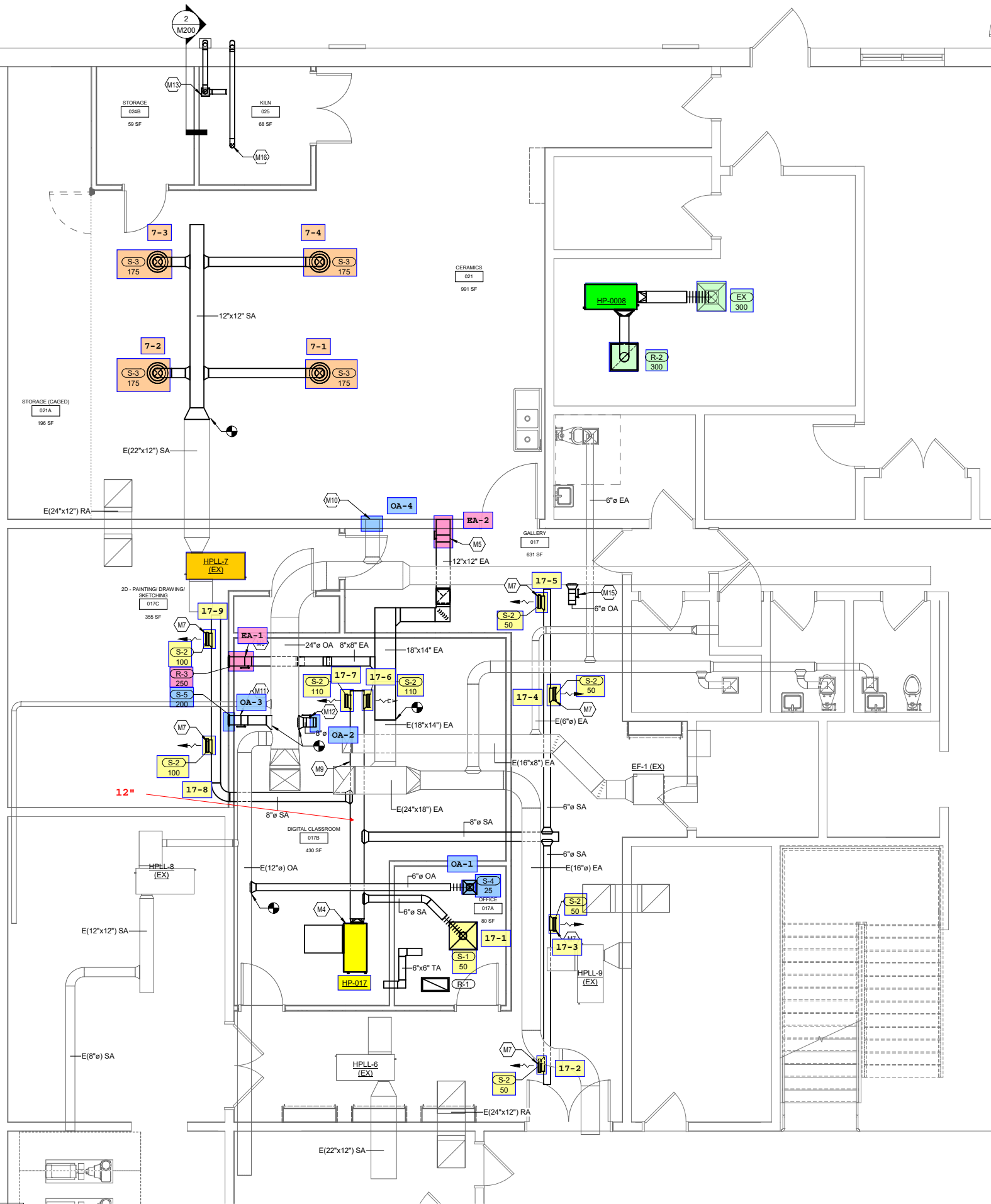
1 MECHANICAL LOWER LEVEL PLAN 1/4" = 1'-0"
