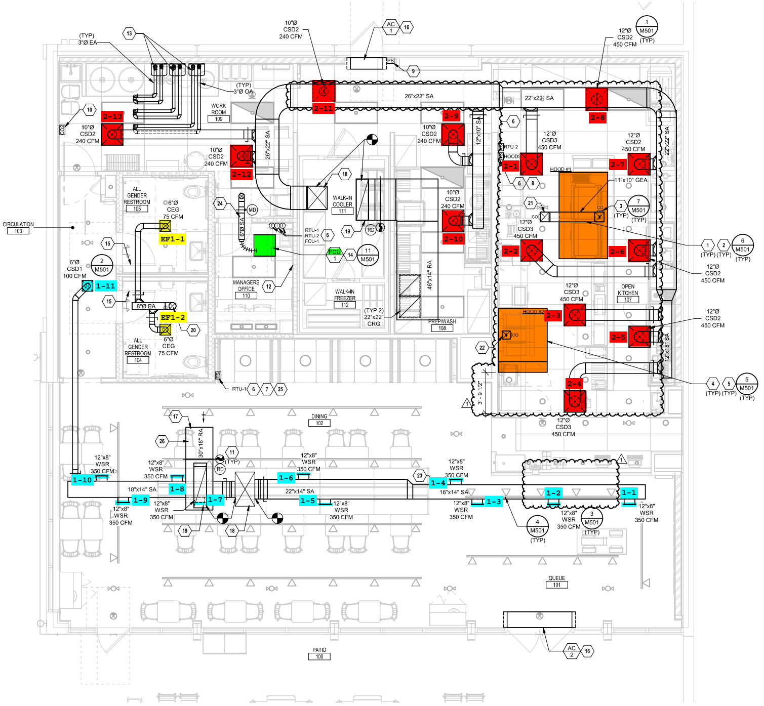
② MECHANICAL FLOOR PLAN 1/4" = 1'-0"
