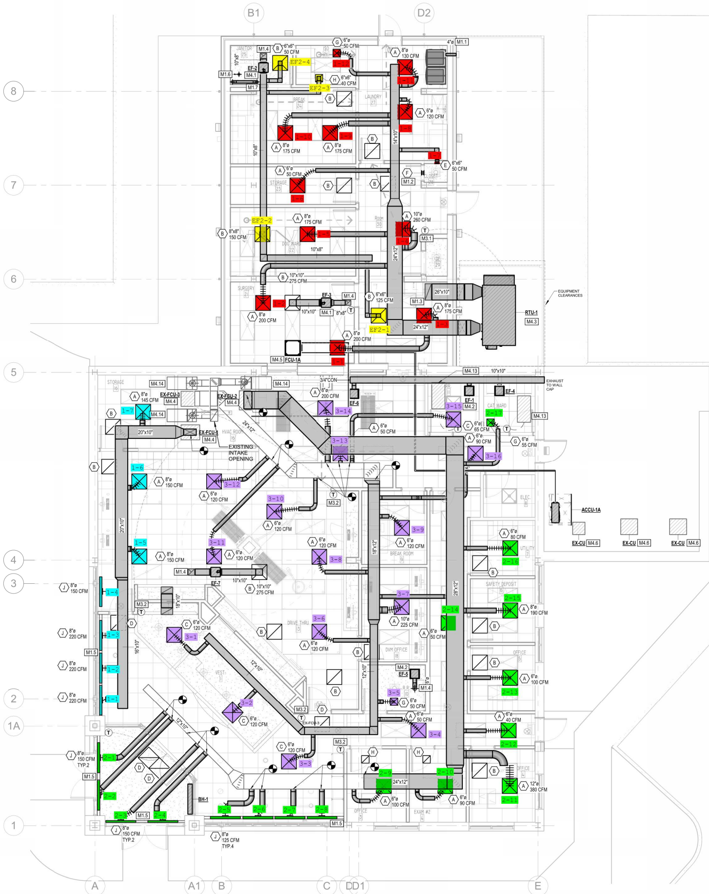
1 LEVEL 1 MECHANICAL PLAN M2.11 3/16" = 1'-0"
