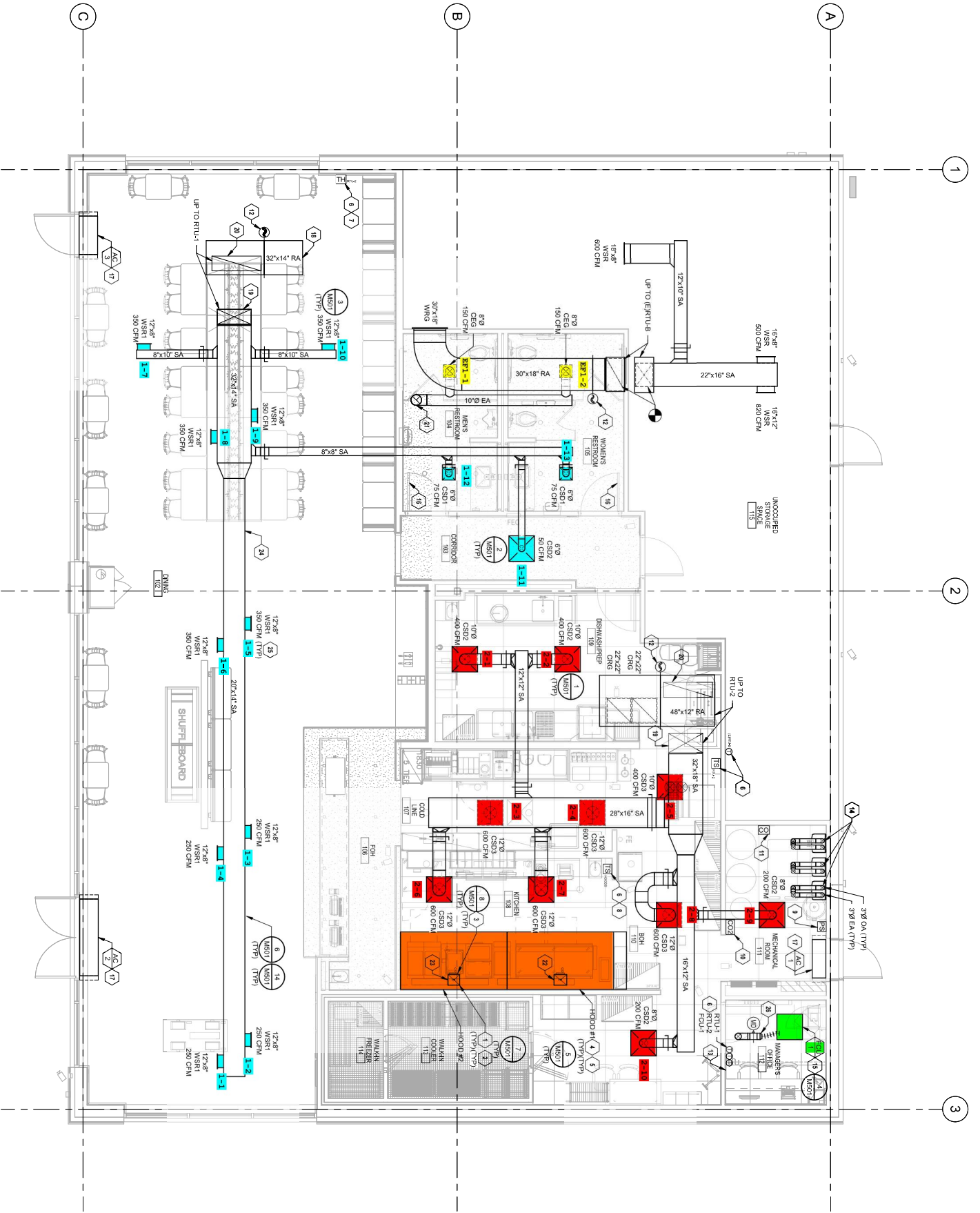
2 MECHANICAL FLOOR PLAN 1/4" = 1'-0"
