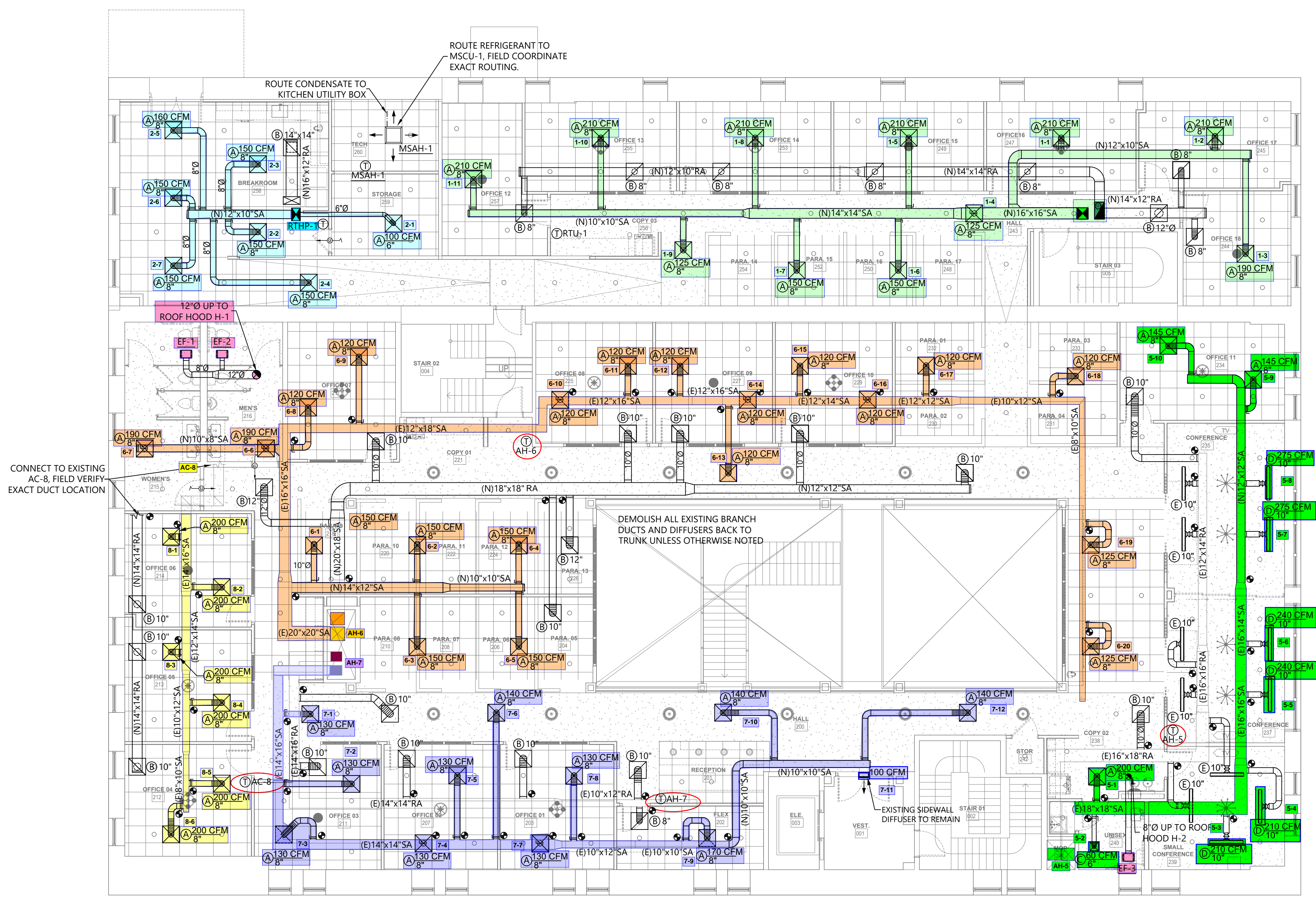
1 MECHANICAL PLAN 1/8" = 1'-0"
