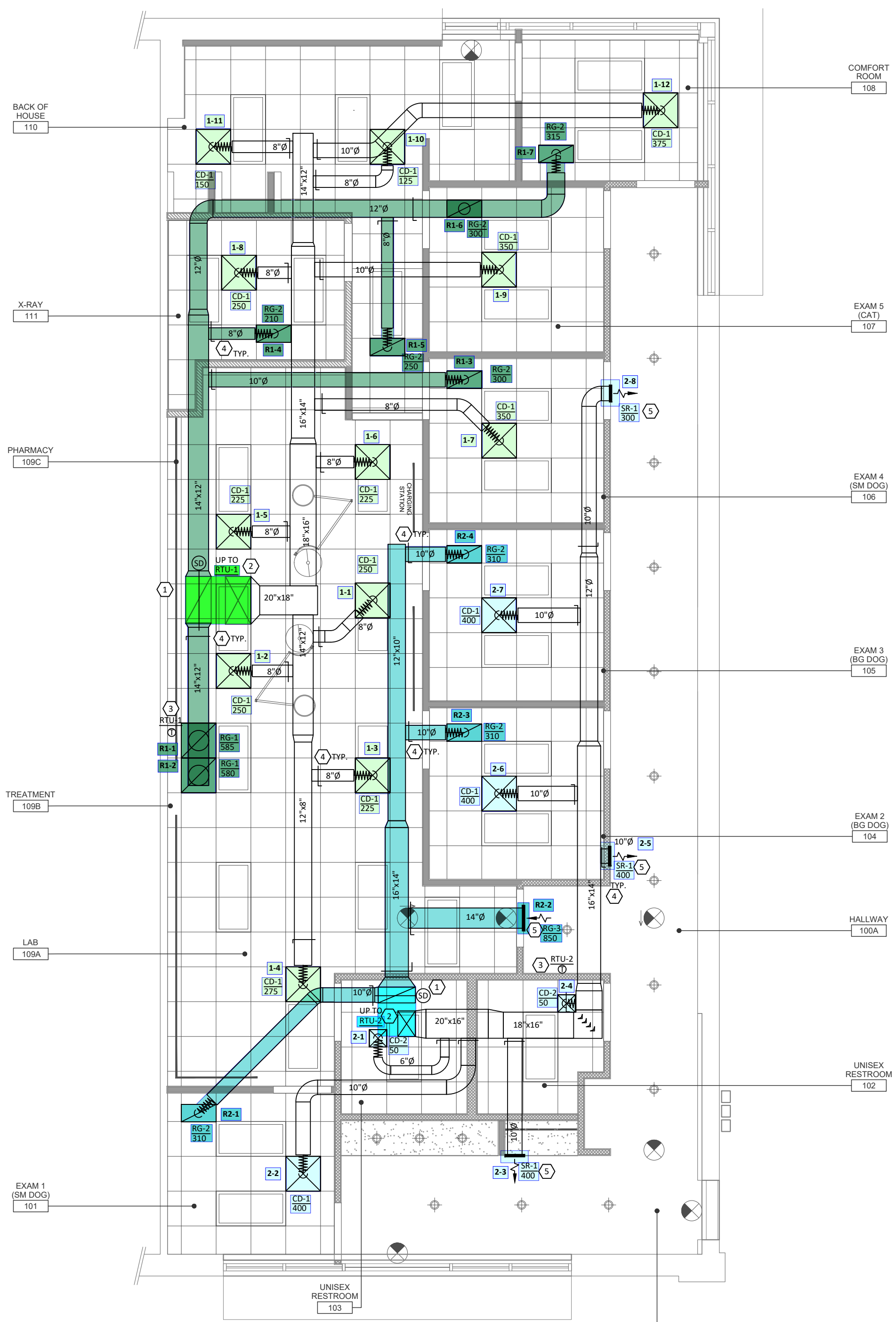
1 MECHANICAL FLOOR PLAN
