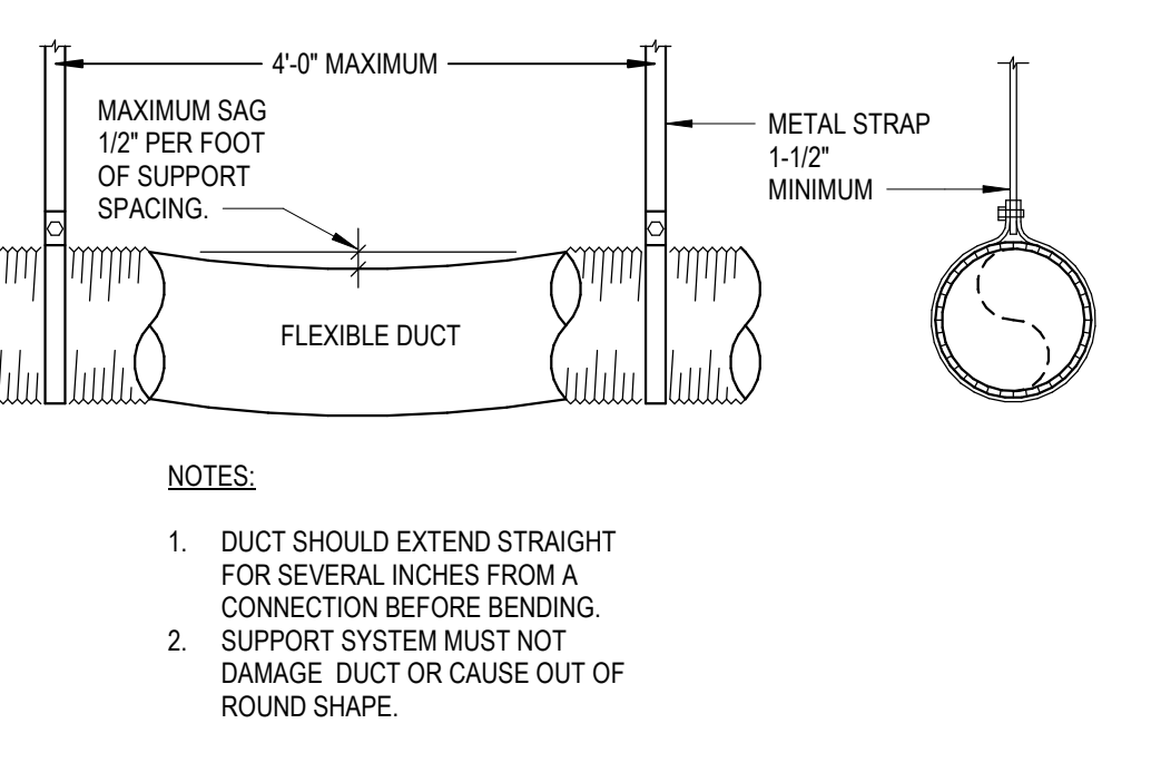
6 FLEX DUCT SUPPORT DETAIL M3.0 NOT TO SCALE
