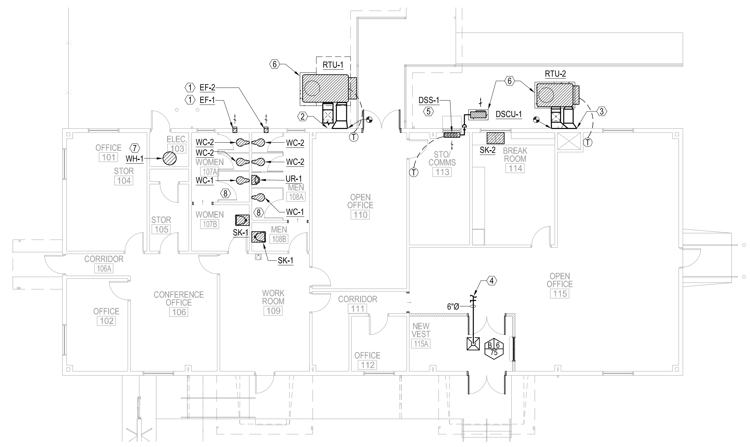
1 BUILDING 525 MECHANICAL PLAN 1/8"=1'-0"
