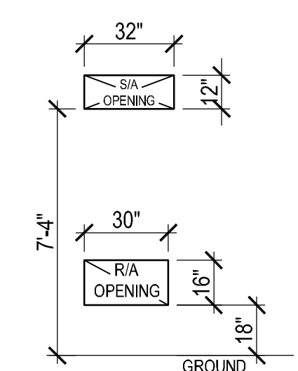
3 BUILDING 525 RTU-2 OPENINGS 1/4"=1'-0"
