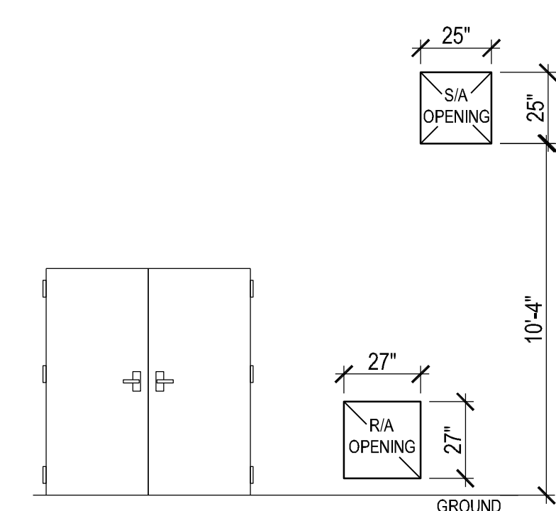
2 BUILDING 525 RTU-1 OPENINGS 1/4"=1'-0"
