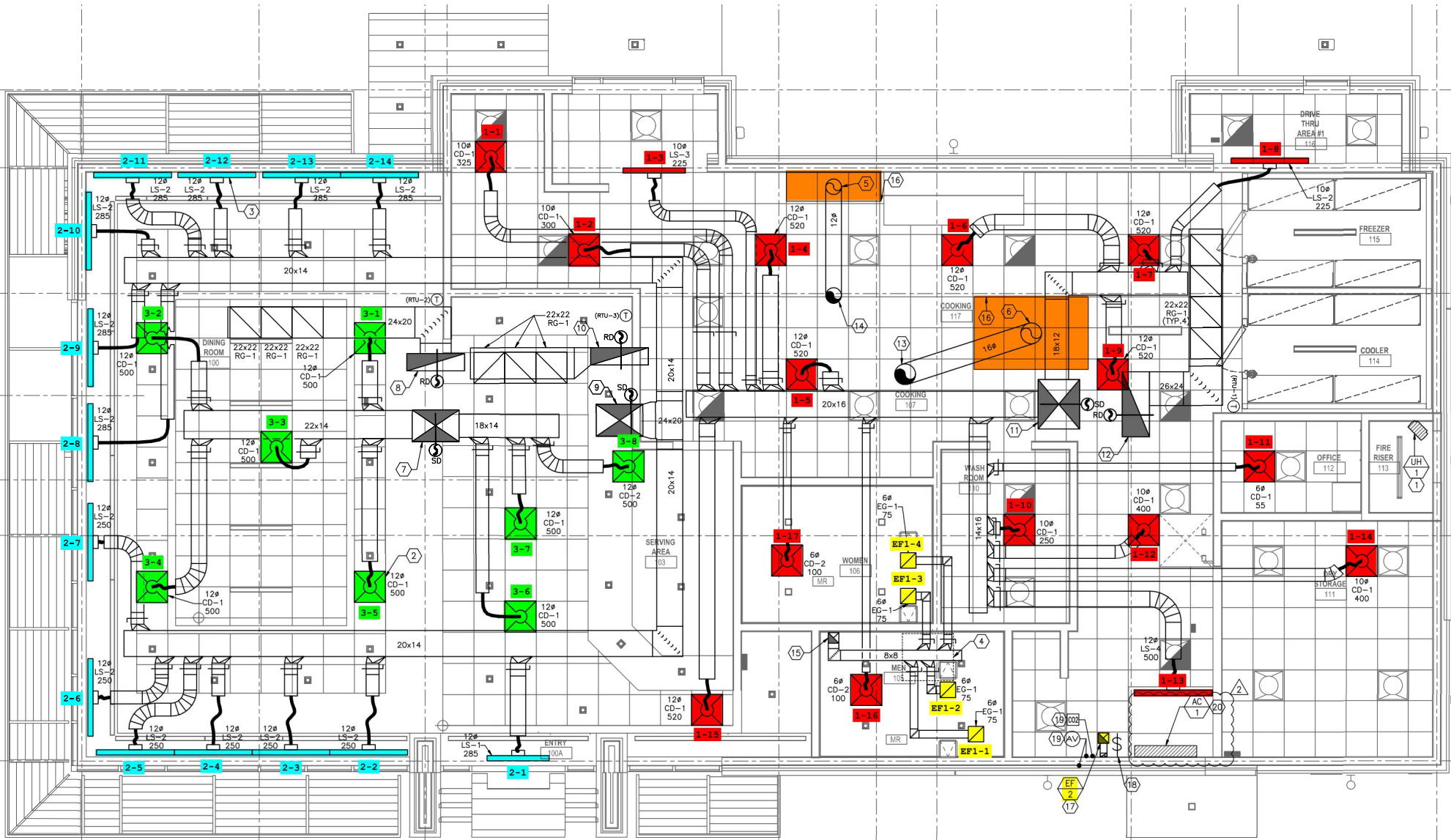
1 MECHANICAL FLOOR PLAN SCALE: 1/4"=1'-0"
