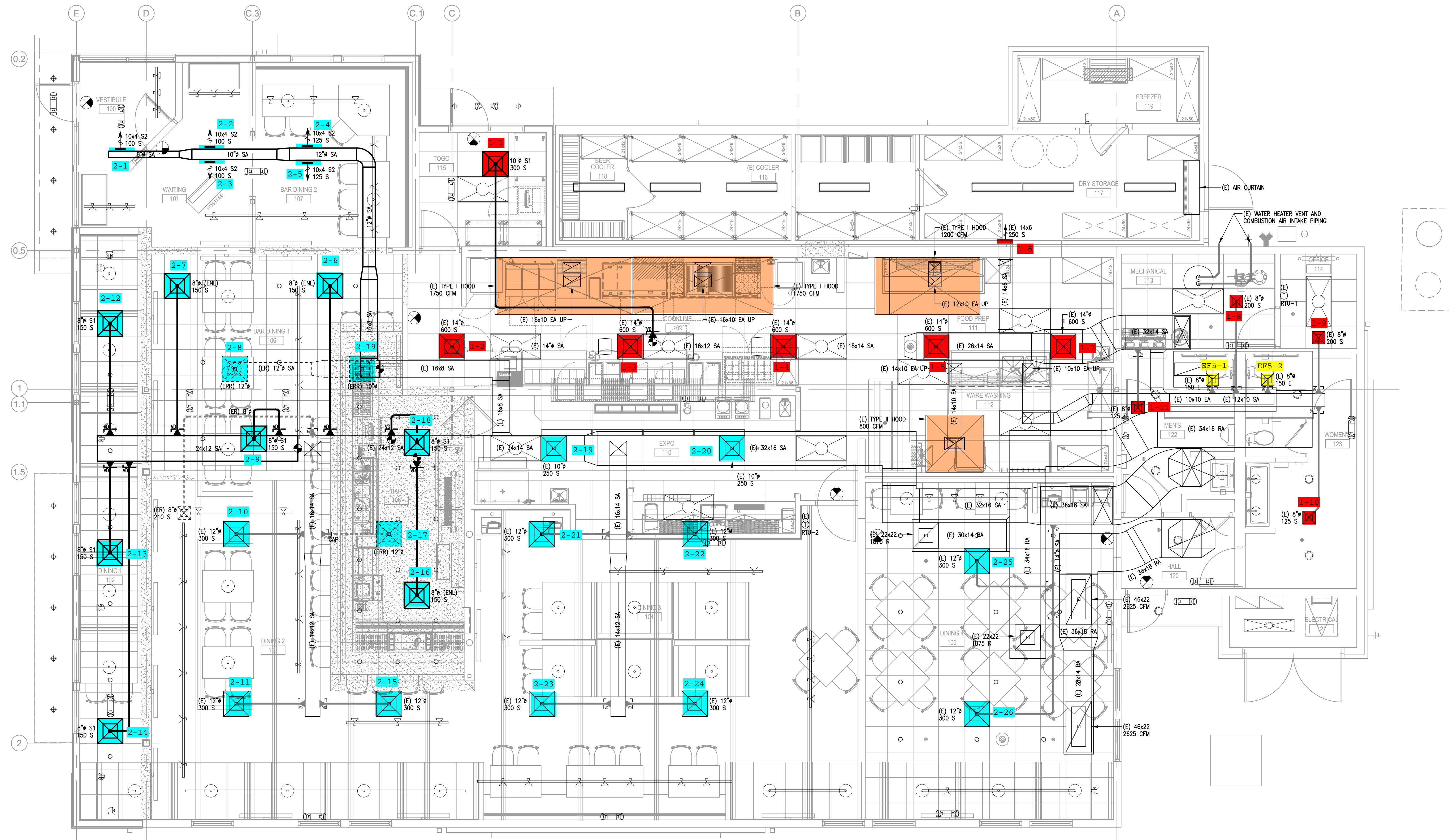
1 FLOOR PLAN - MECHANICAL VENTILATION 1/4" = 1'-0"
