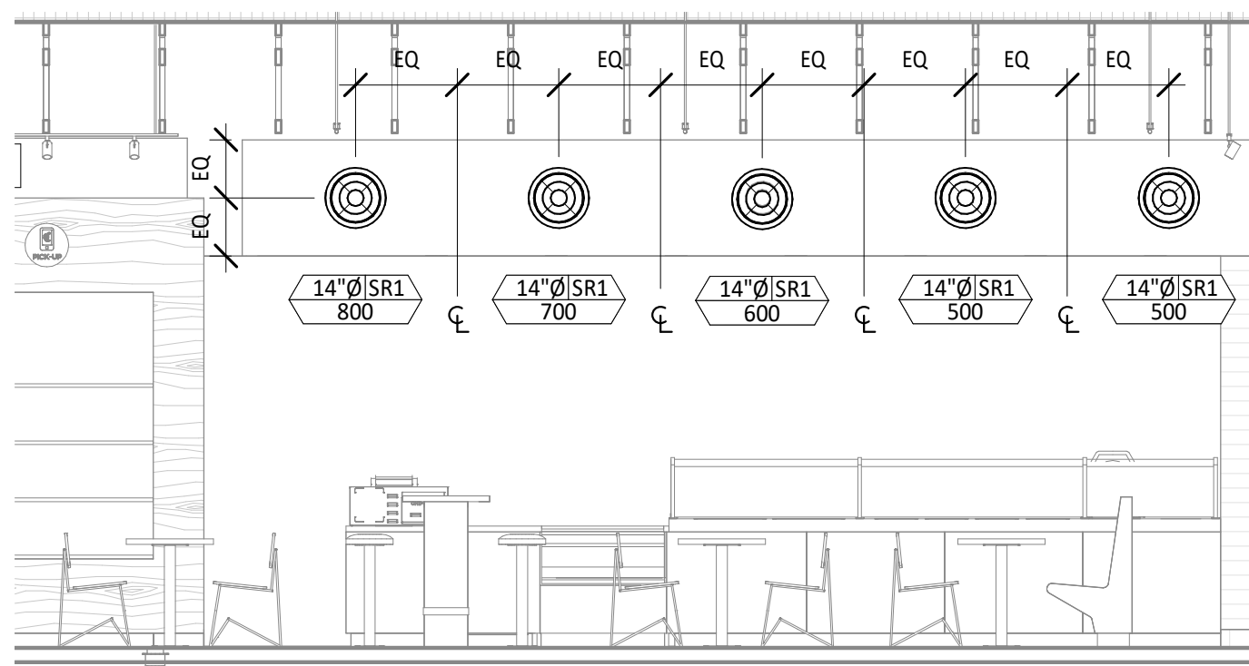
9 HVAC DINING ROOM SECTION 1/4" = 1'-0"
