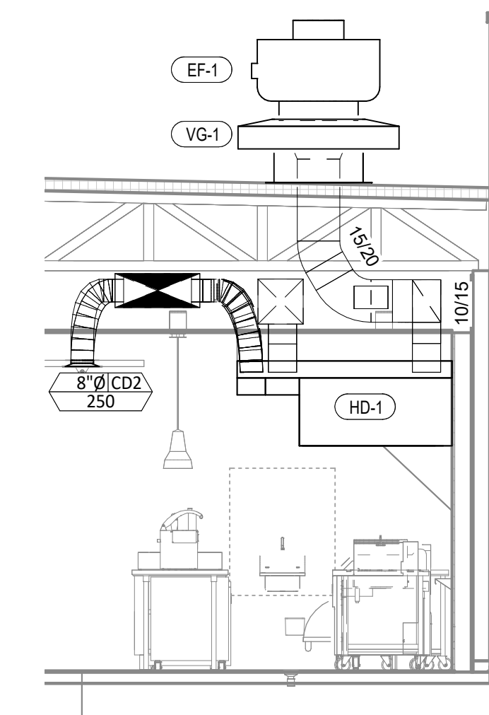
7 DUCT SECTION AT HOOD 1/4" = 1'-0"
