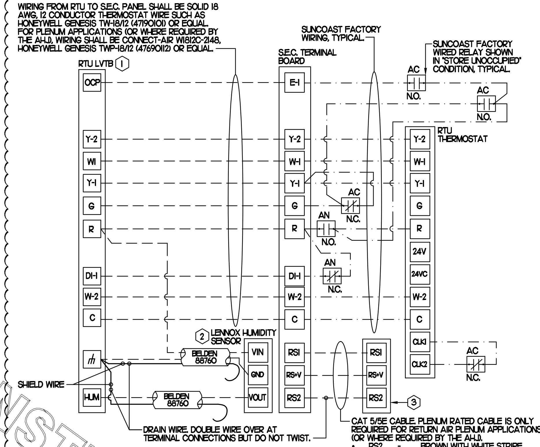
2 ROOFTOP UNIT CONTROL WIRING - LENNOX NONE
