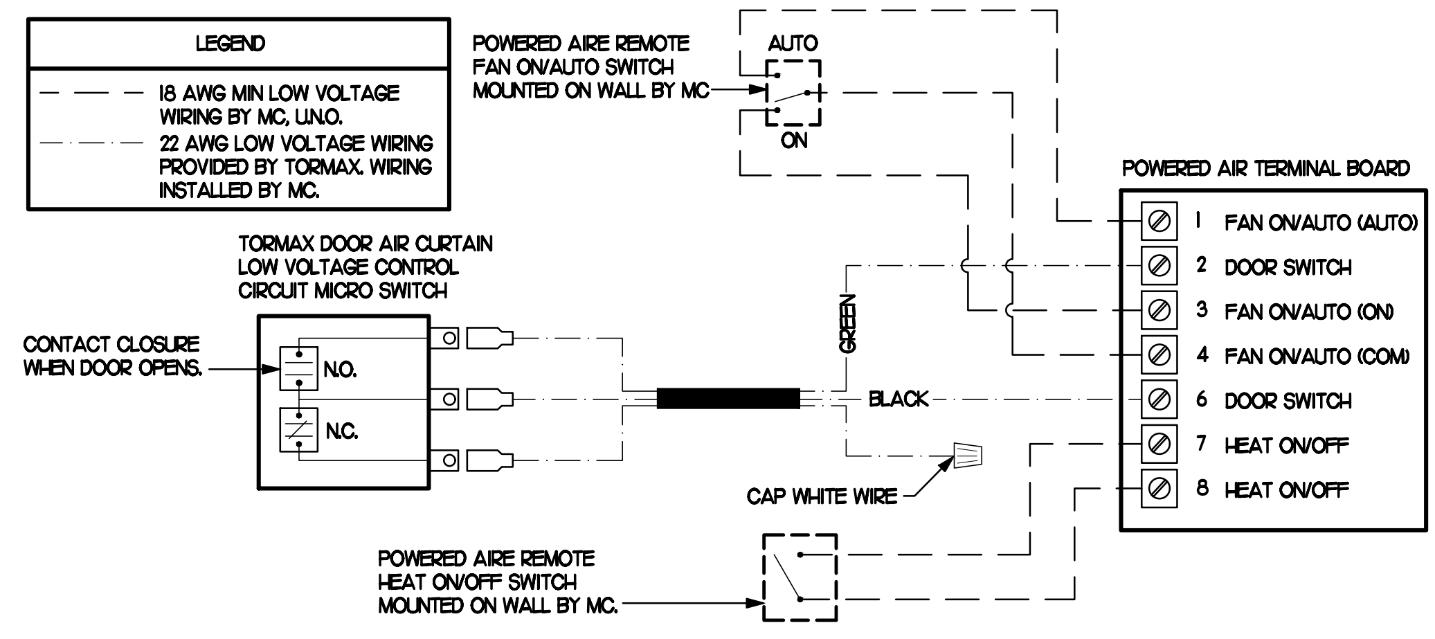
4 AIR CURTAIN WIRING DIAGRAM NO SCALE
