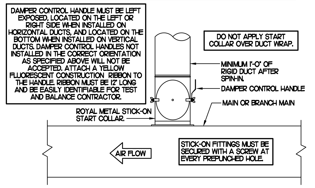
2 START COLLAR NO SCALE
