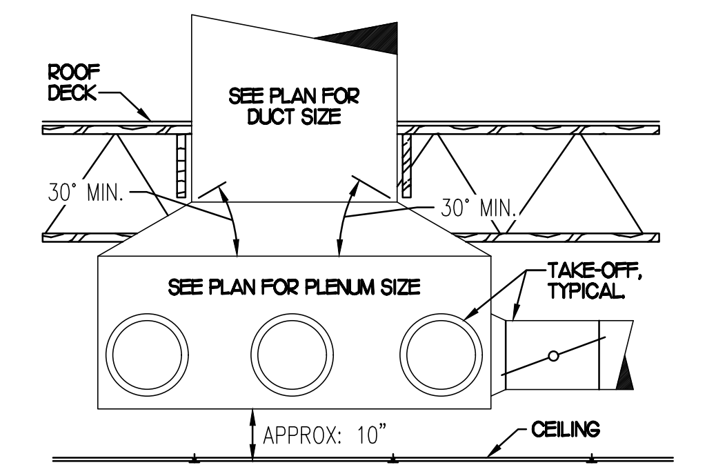
5 RETURN DROP GEOMETRY NO SCALE
