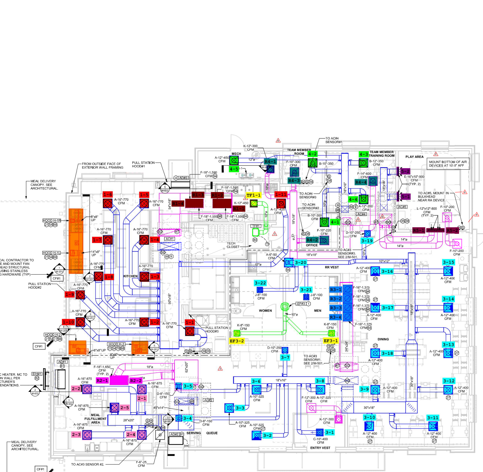
1 EQUIPMENT AND DUCTWORK PLAN 1/4" = 1'-0"
