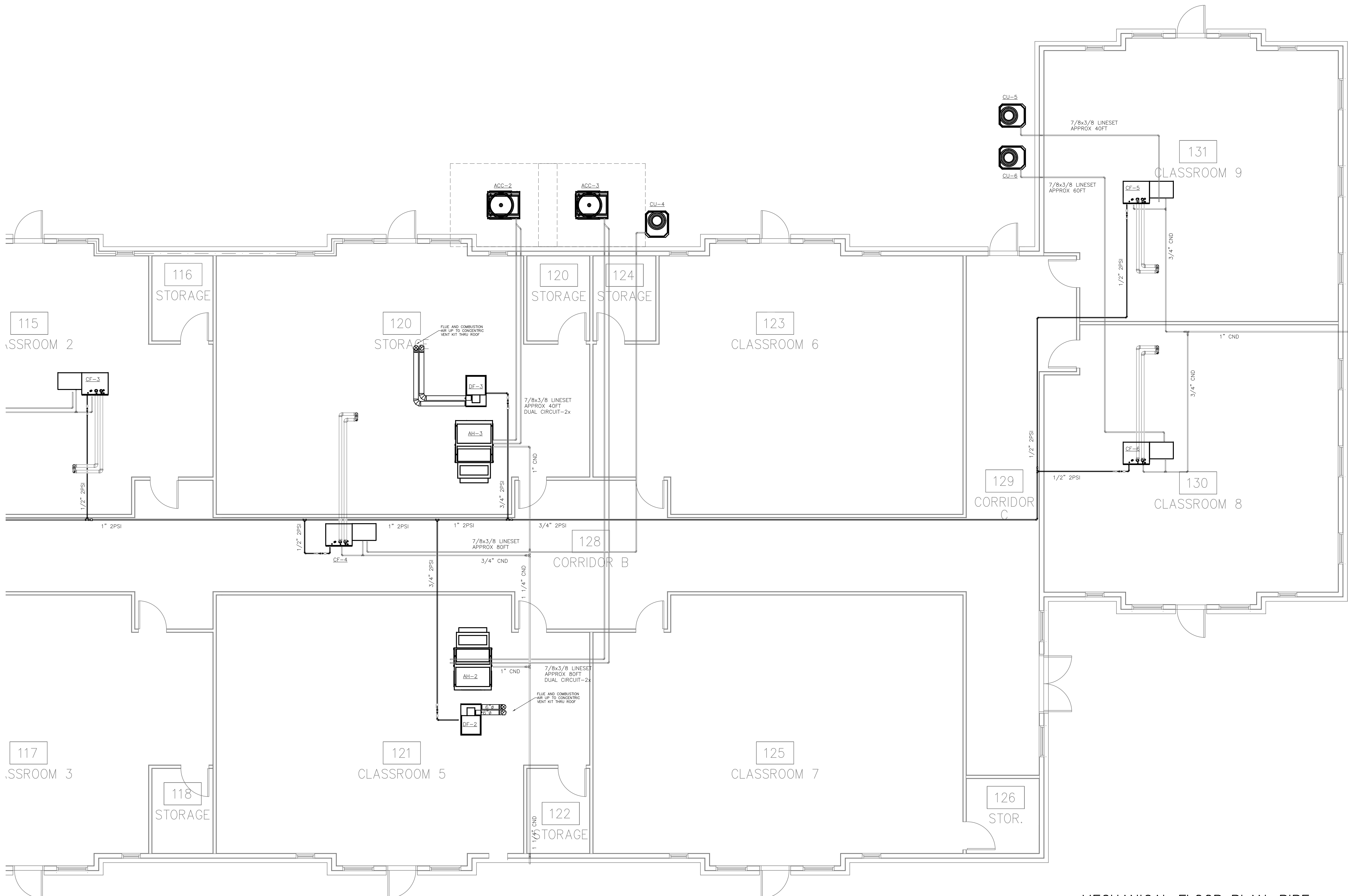
MECHANICAL FLOOR PLAN-PIPE SCALE: 1/4"=1'-0"
