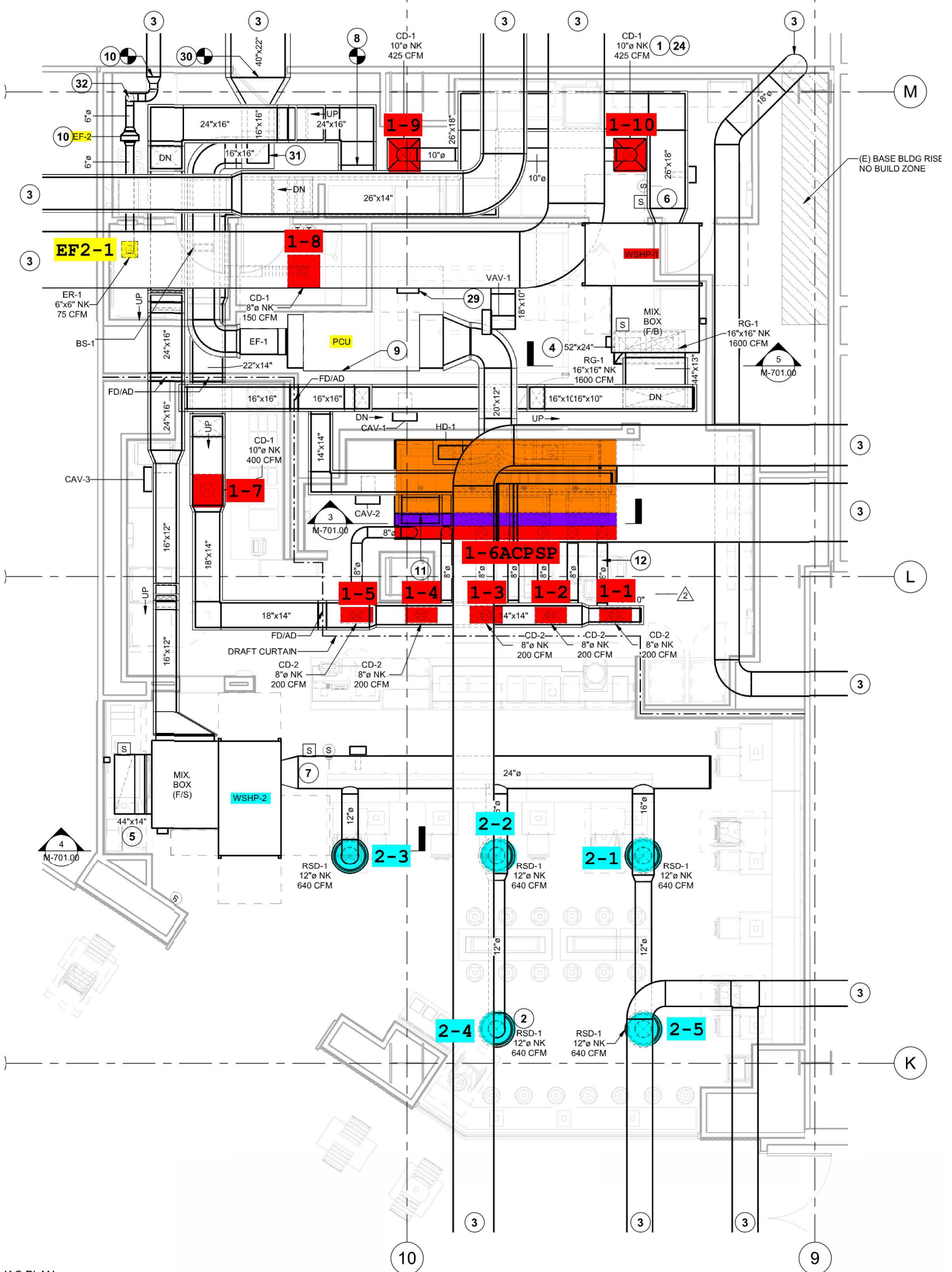
'AC PLAN 4" = 1'-0"
