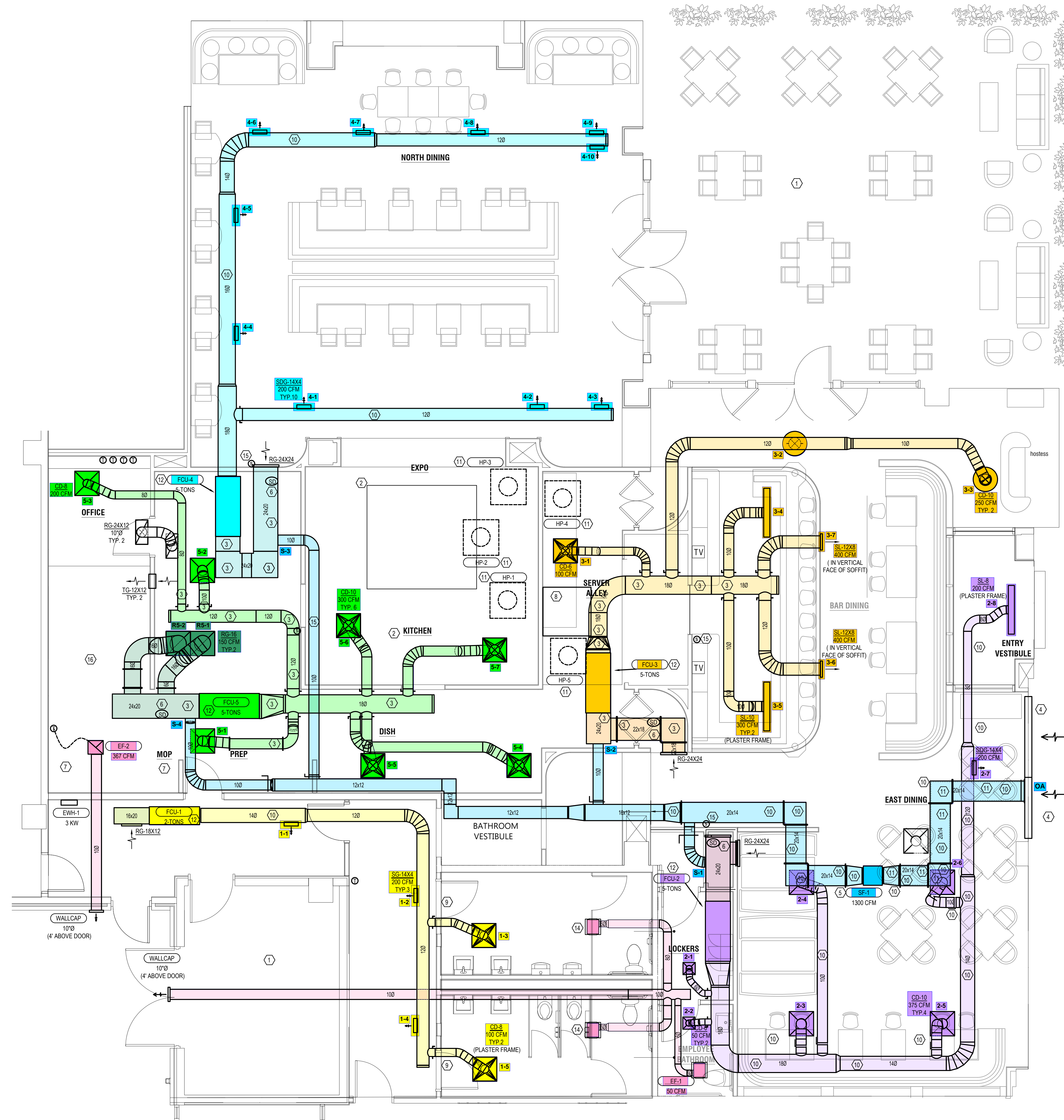
SECOND FLOOR HVAC PLAN SCALE: 1/4" = 1'-0"
