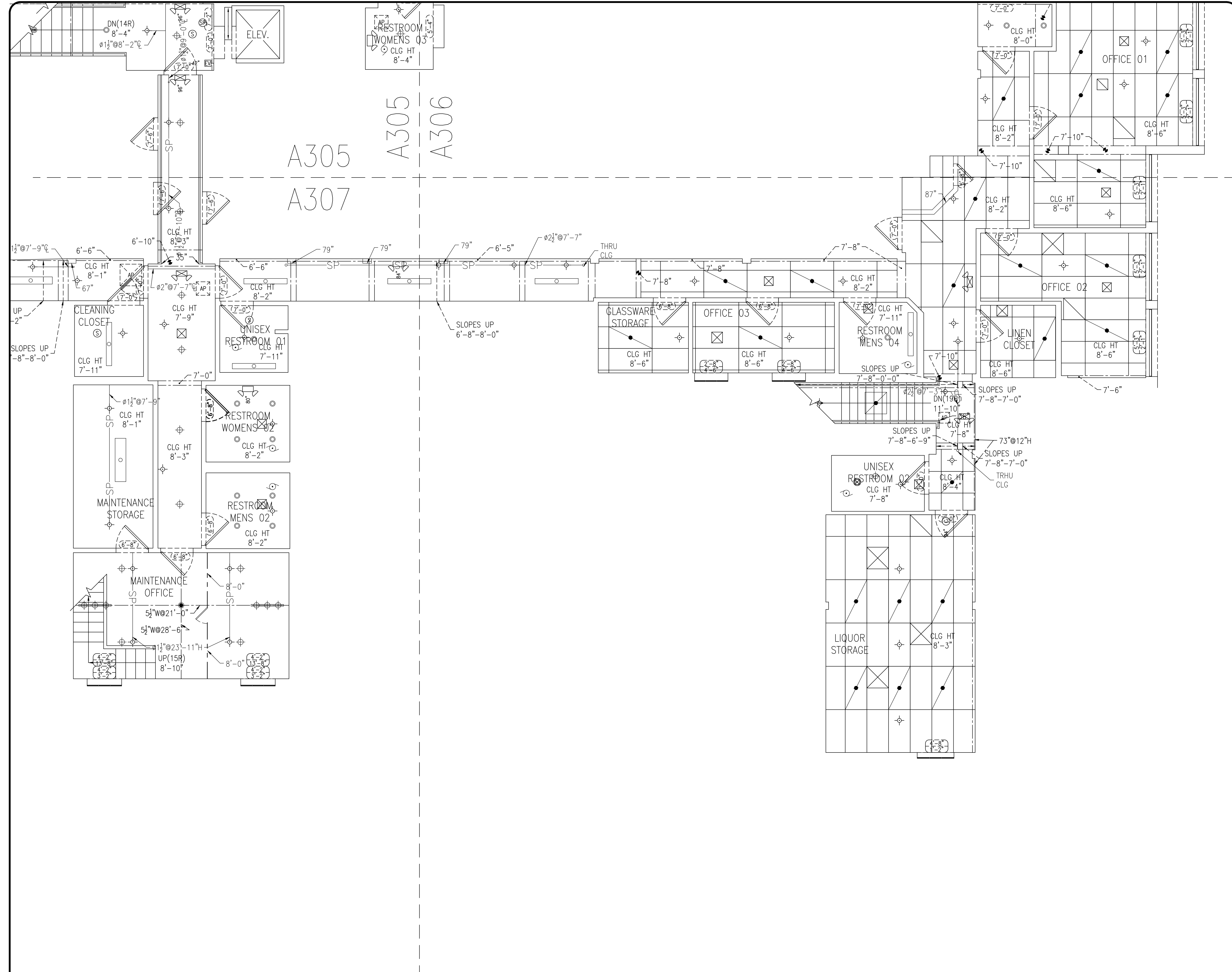
2ND LEVEL REFLECTED CEILING PLAN-3
