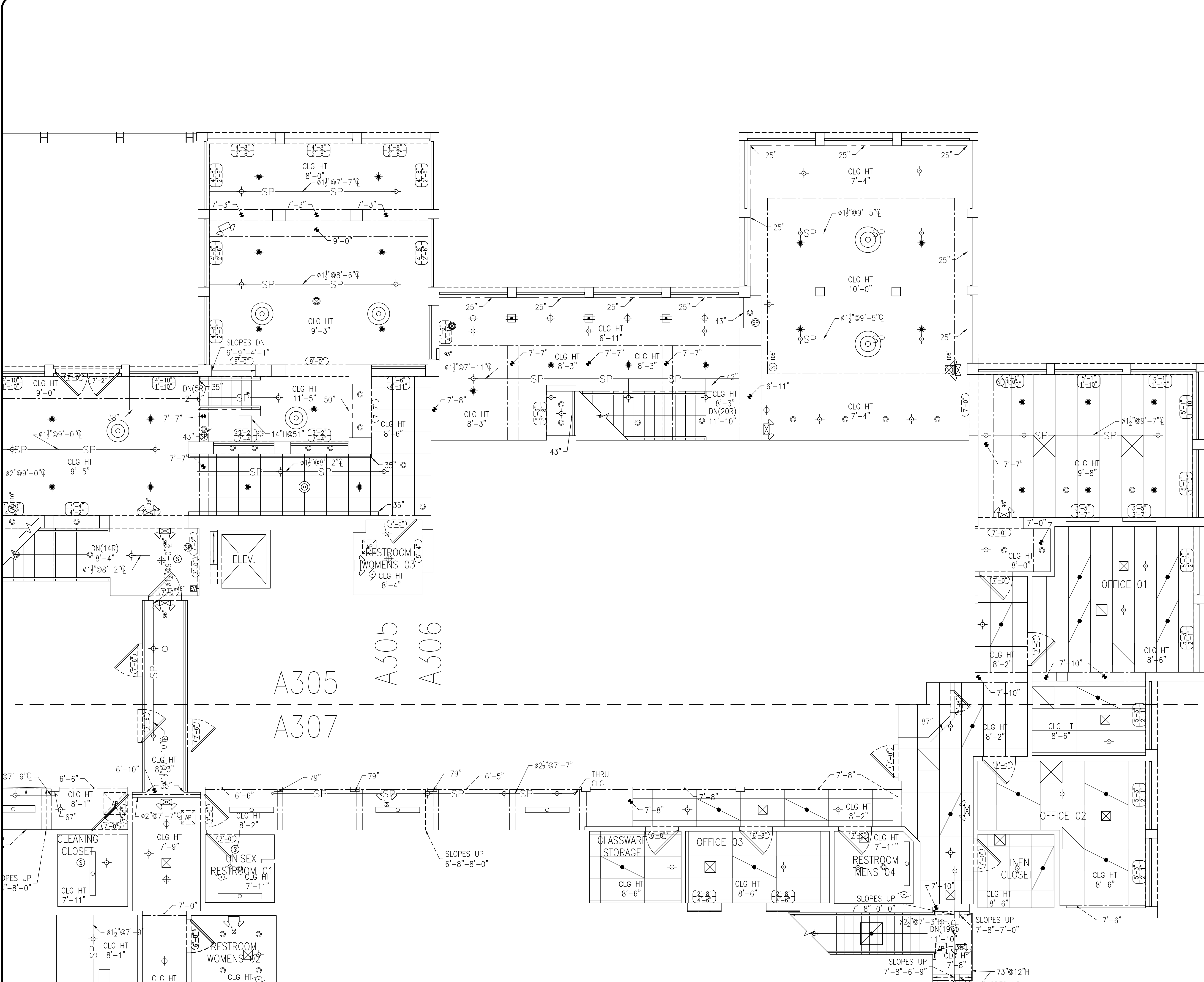
2ND LEVEL REFLECTED CEILING PLAN-2
