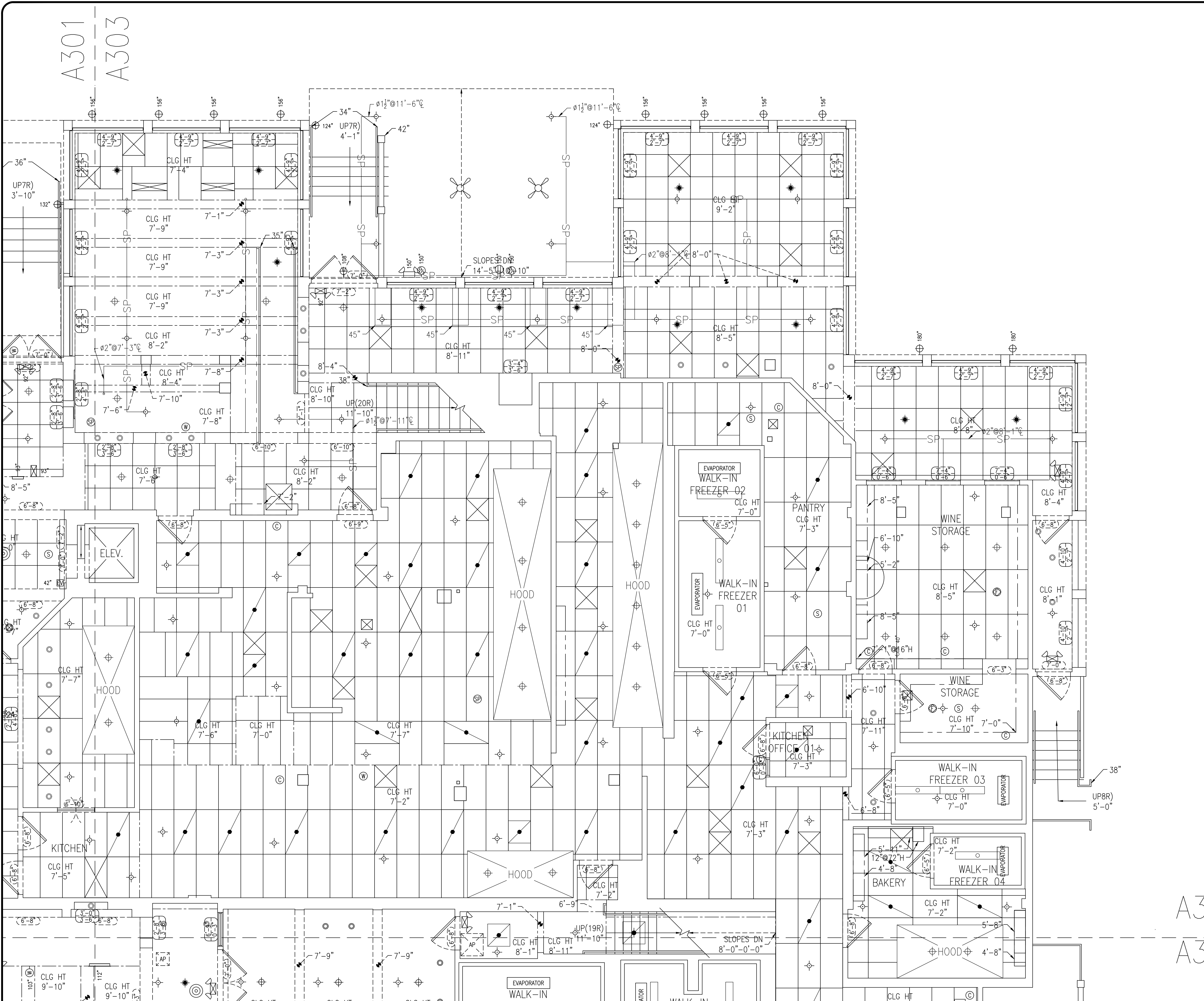
1ST LEVEL REFLECTED CEILING PLAN-3
