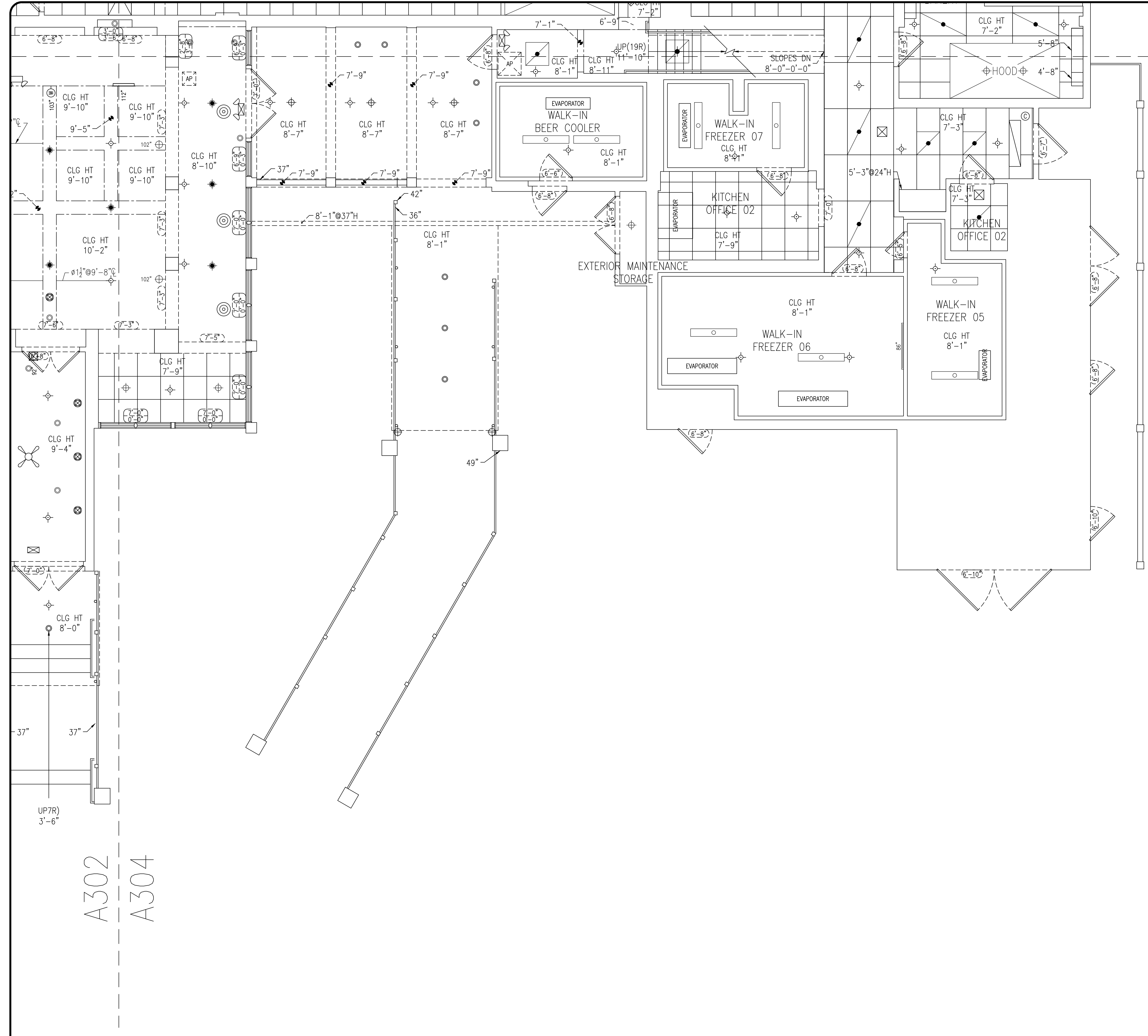
1ST LEVEL REFLECTED CEILING PLAN-4
