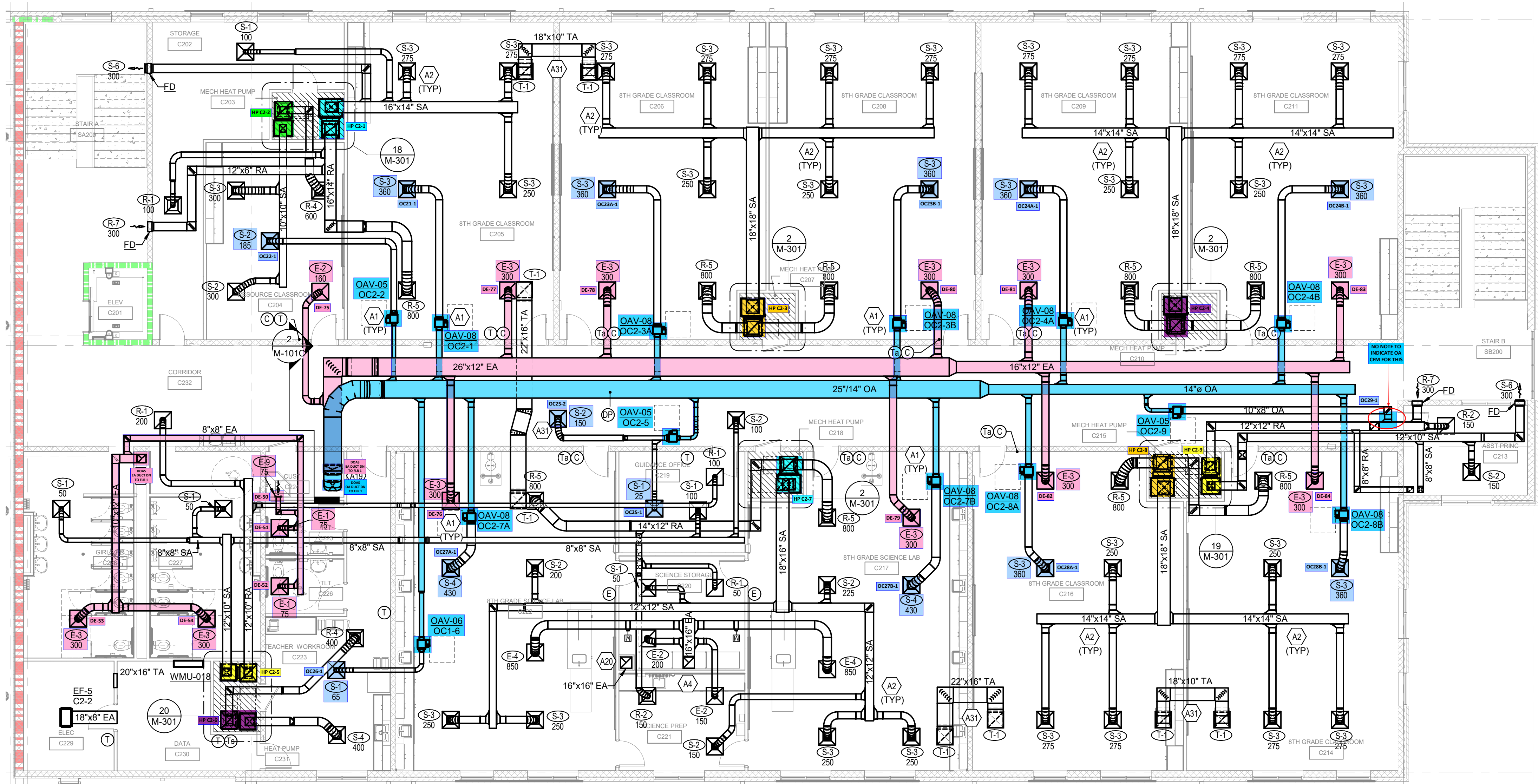
① SECOND FLOOR PLAN - AIR DISTRIBUTION - AREA C 1/8" = 1'-0"
