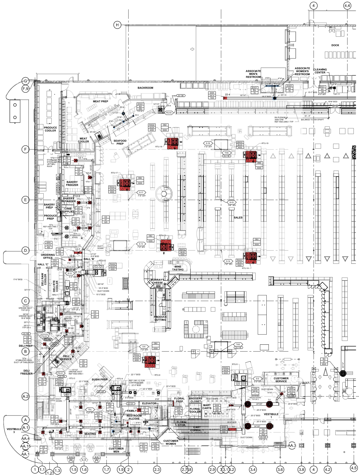
1 HVAC PLAN - EAST 332' x 141'
