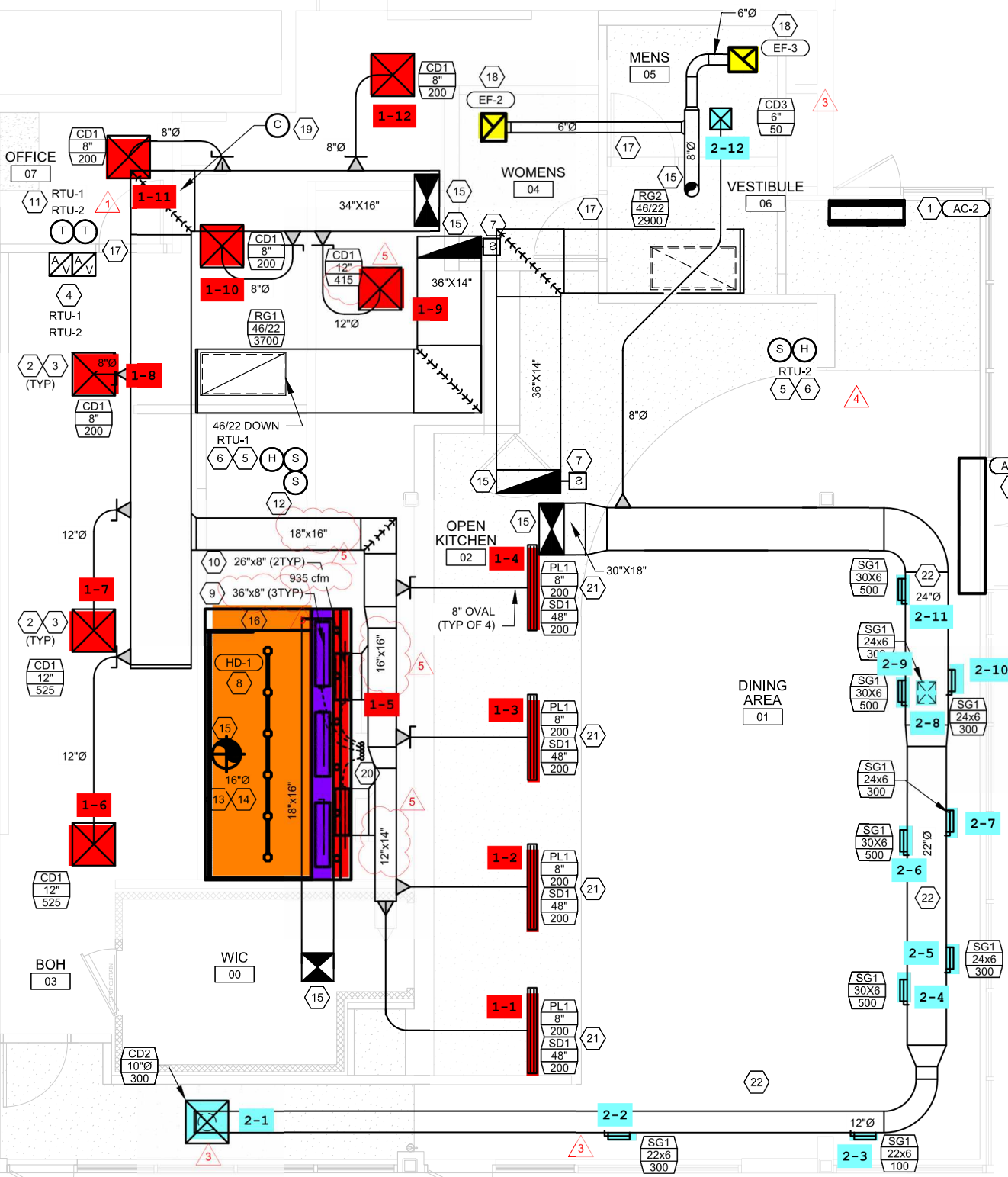
1 MECHANICAL PLAN 1/4" = 1'-0"
