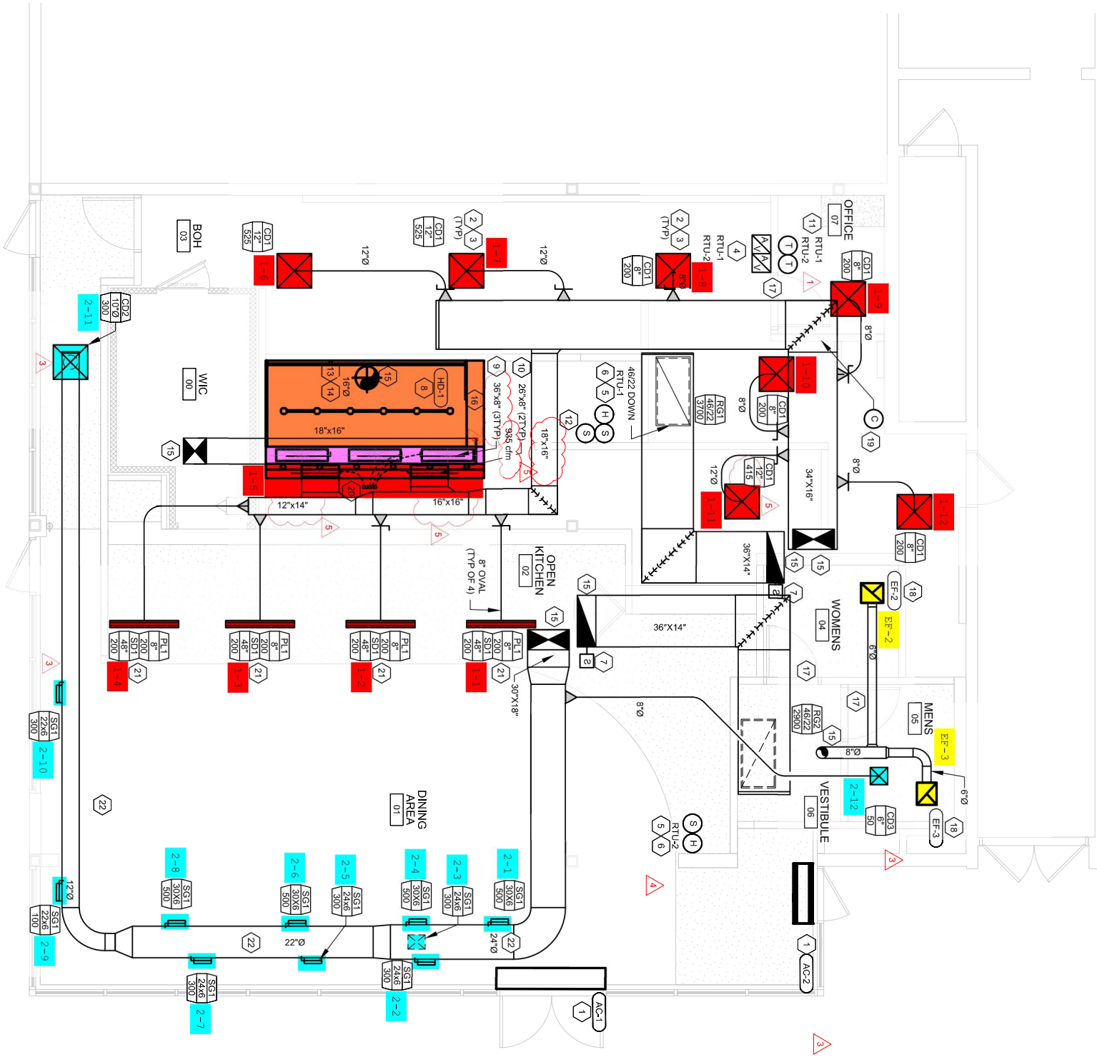
1 MECHANICAL PLAN 1/4" = 1'-0"
