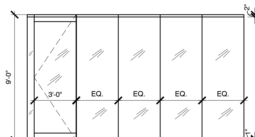
H BUILDING STANDARD TEMPERED GLASS DOOR W/4" CONT. HEAD & SHOE LEADING EDGE OF BOTTOM RAIL TO BE TAPERED 60" MINIMUM FROM HORIZONTAL AND SIDELIGHT IN EXPOSED U-CHANNELS
