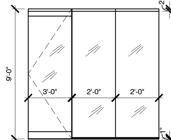
C BUILDING STANDARD TEMPERED GLASS DOOR W/4" CONT. HEAD & SHOE LEADING EDGE OF BOTTOM RAIL TO BE TAPERED 60" MINIMUM FROM HORIZONTAL AND SIDELIGHT IN EXPOSED U-CHANNELS
