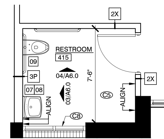
02 ENLARGED RESTROOM PLAN SCALE: 1/8" = 1'-0"
