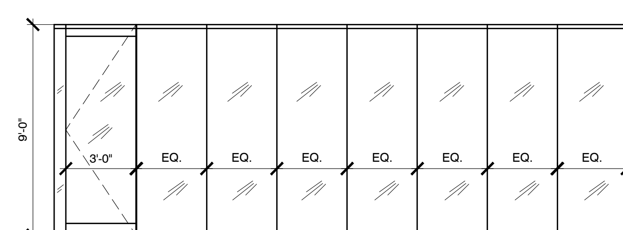
I BUILDING STANDARD TEMPERED GLASS DOOR W/4" CONT. HEAD & SHOE LEADING EDGE OF BOTTOM RAIL TO BE TAPERED 60" MINIMUM FROM HORIZONTAL AND SIDELIGHT IN EXPOSED U-CHANNELS
