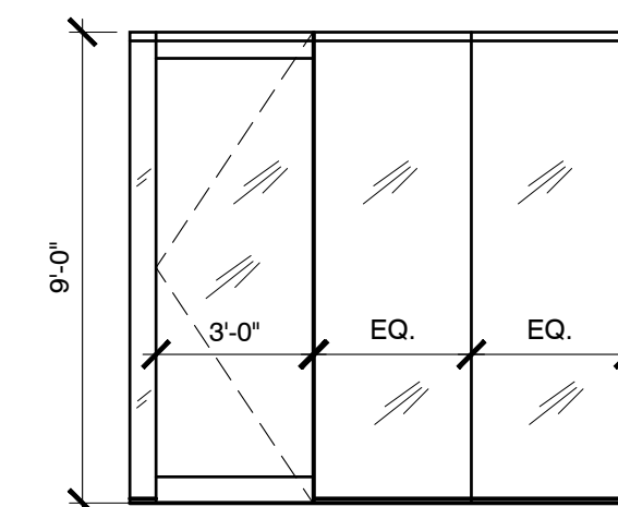
F BUILDING STANDARD TEMPERED GLASS DOOR W/4" CONT. HEAD & SHOE LEADING EDGE OF BOTTOM RAIL TO BE TAPERED 60" MINIMUM FROM HORIZONTAL AND SIDELIGHT IN EXPOSED U-CHANNELS
