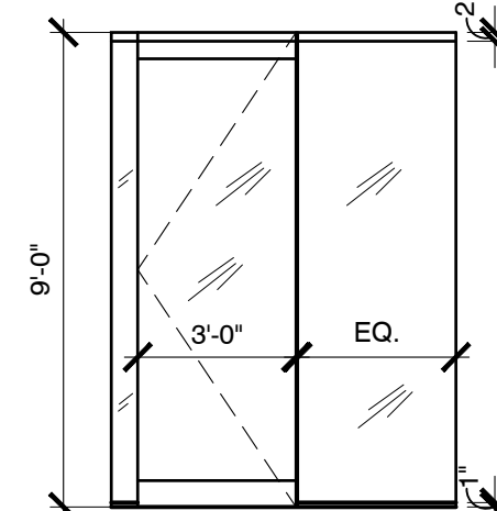
D BUILDING STANDARD TEMPERED GLASS DOOR W/4" CONT. HEAD & SHOE LEADING EDGE OF BOTTOM RAIL TO BE TAPERED 60" MINIMUM FROM HORIZONTAL AND SIDELIGHT IN EXPOSED U-CHANNELS
