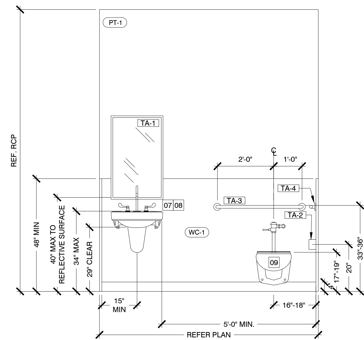
03 ELEVATION @ RESTROOM SCALE: 1/2" = 1'-0"
