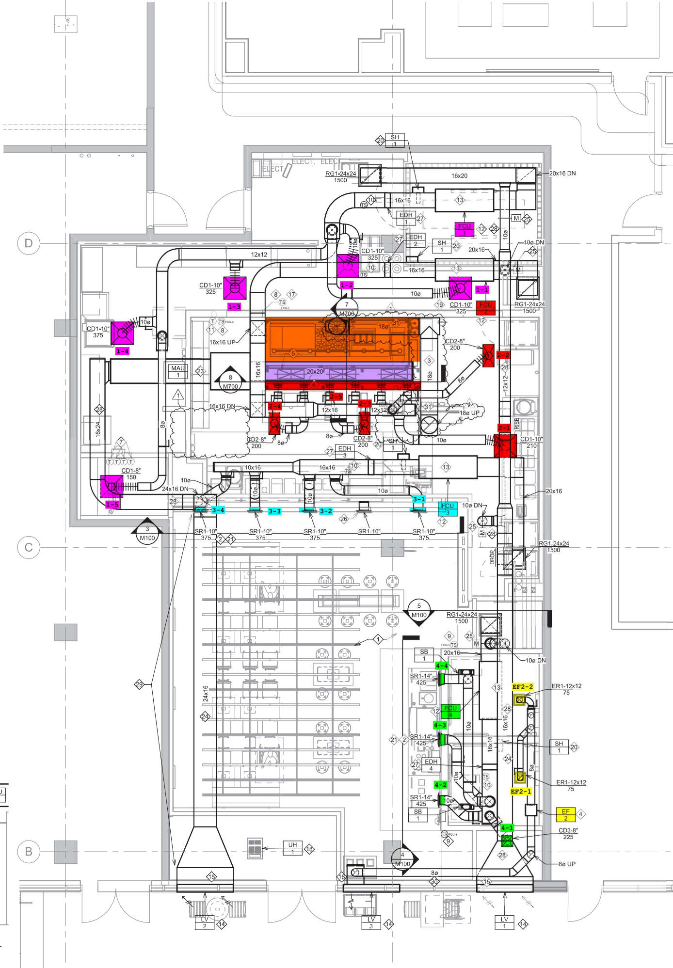
① HVAC FLOOR PLAN 1/4" = 1'-0"
