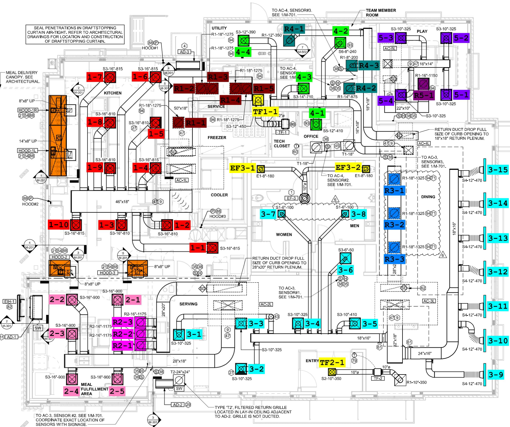
1 EQUIPMENT AND DUCTWORK PLAN 1/4" = 1'-0"
