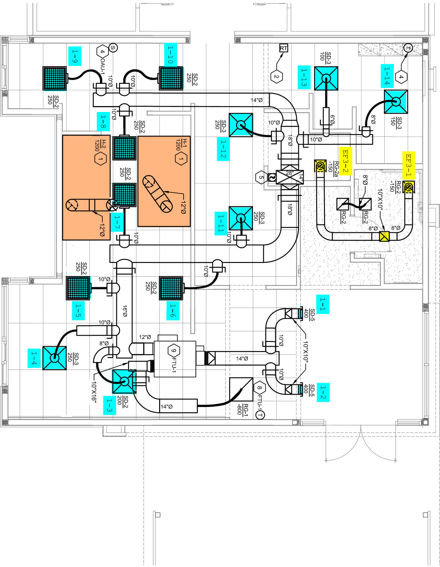
MECHANICAL PLAN 1
