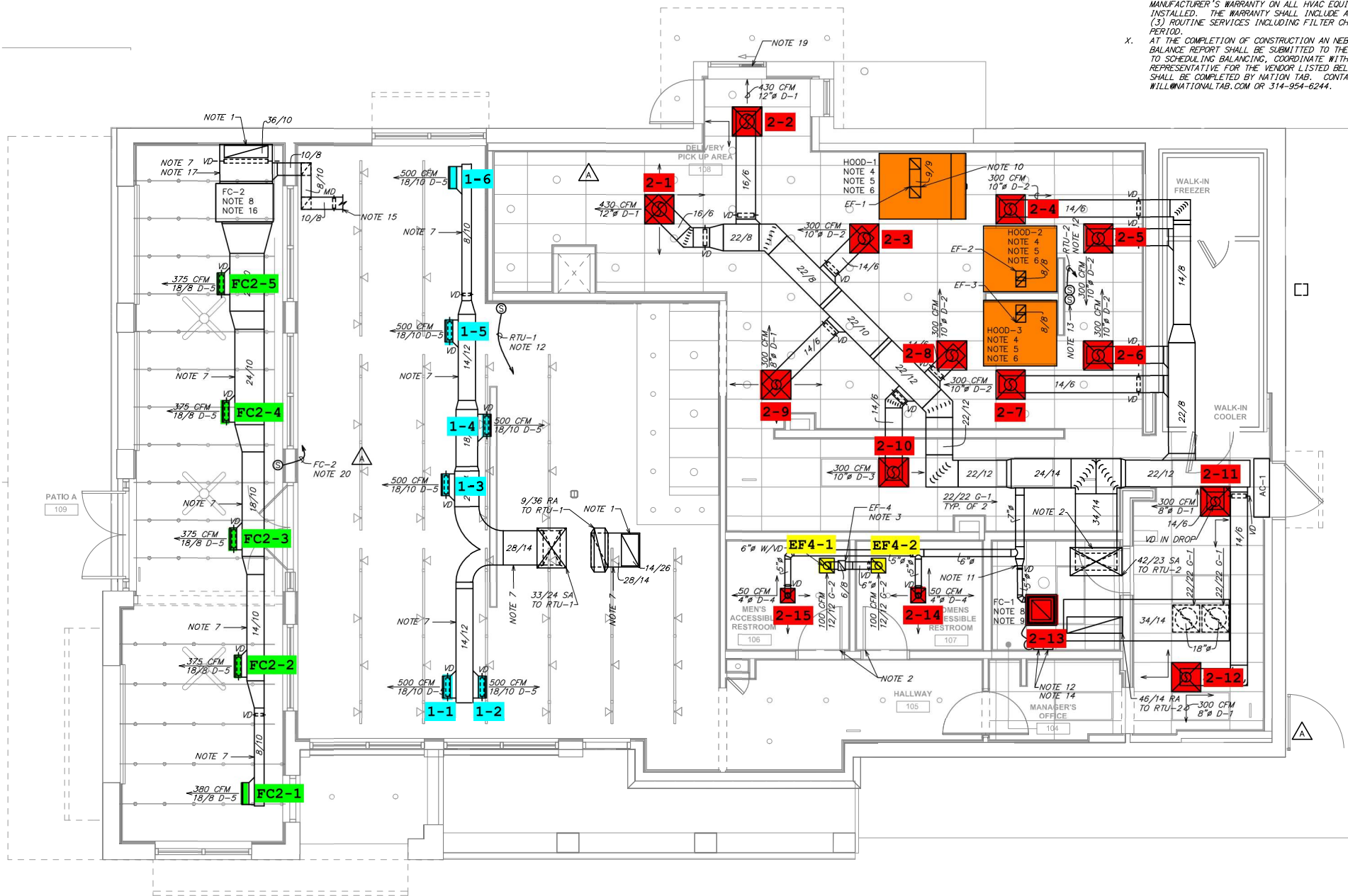
1 MECHANICAL FLOOR PLAN SCALE: 1/4" = 1'-0"
