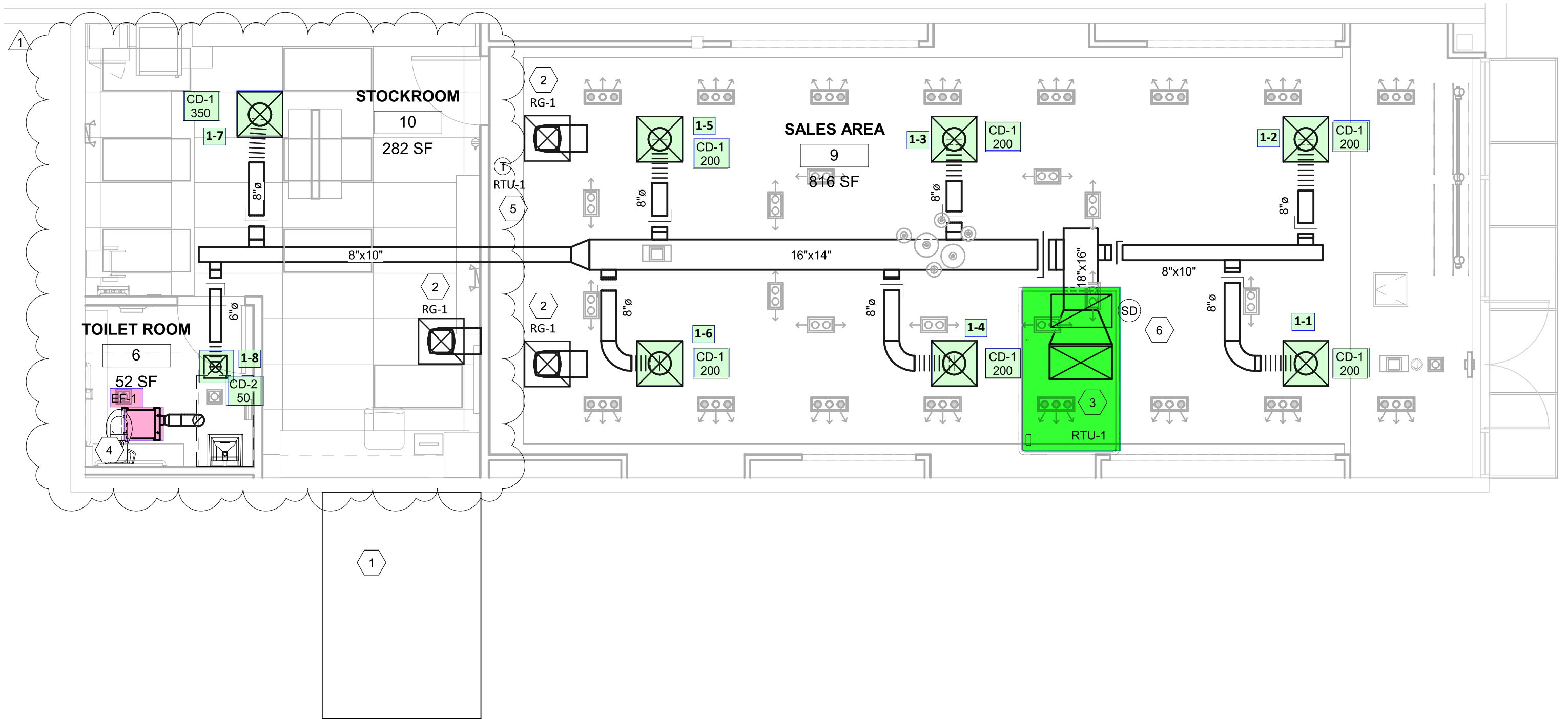
1 MECHANICAL PLAN M101 1/4" = 1'-0"
