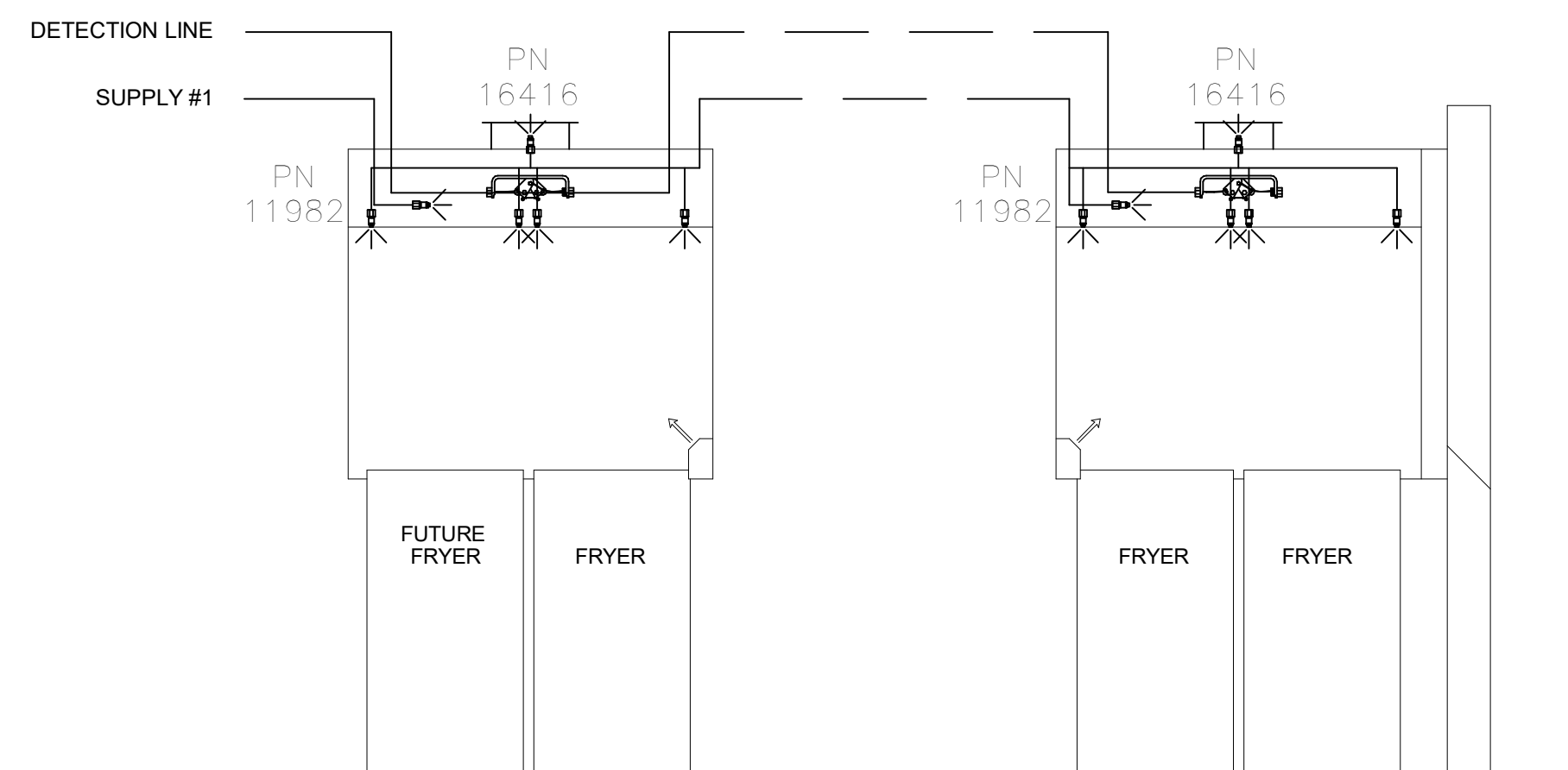
AMEREX FIRE SYSTEM LAYOUT
