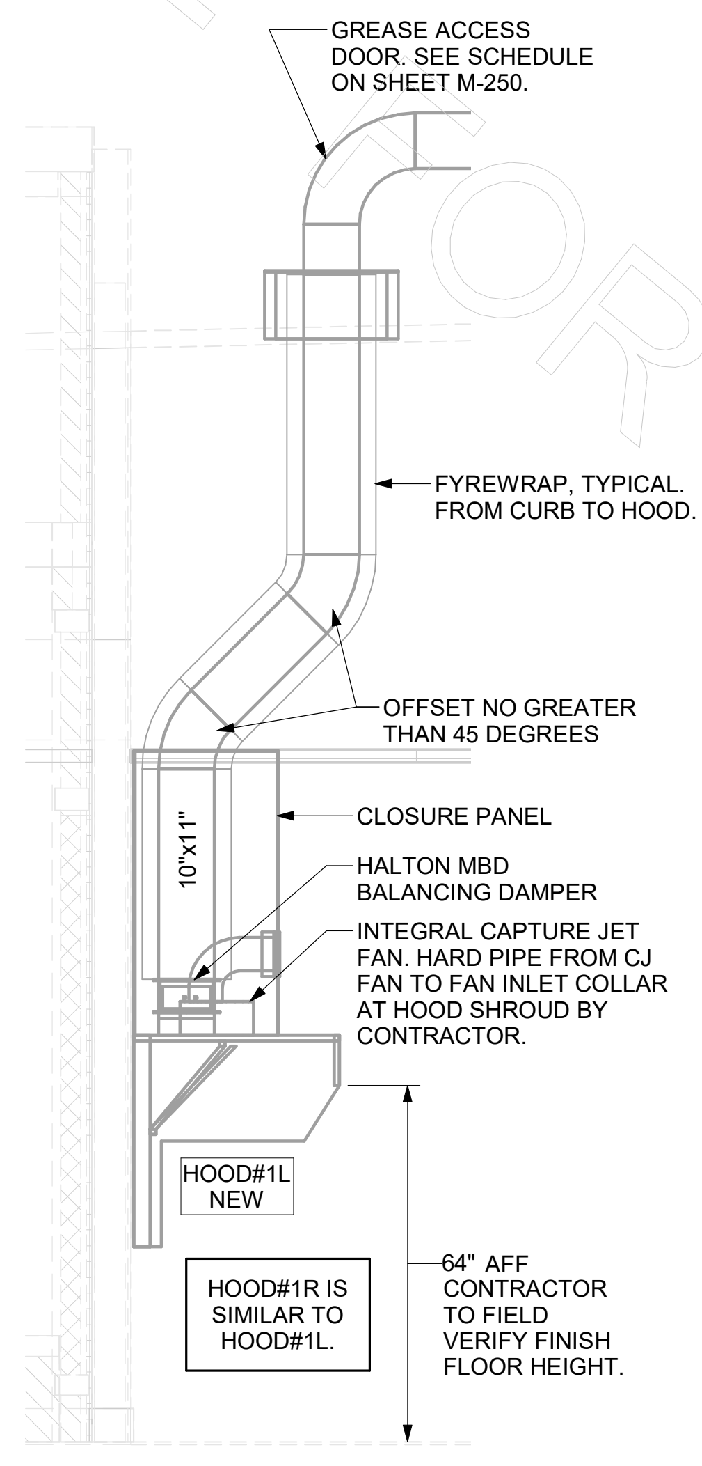
3 HOOD#1 SIDE ELEVATION NOT TO SCALE
