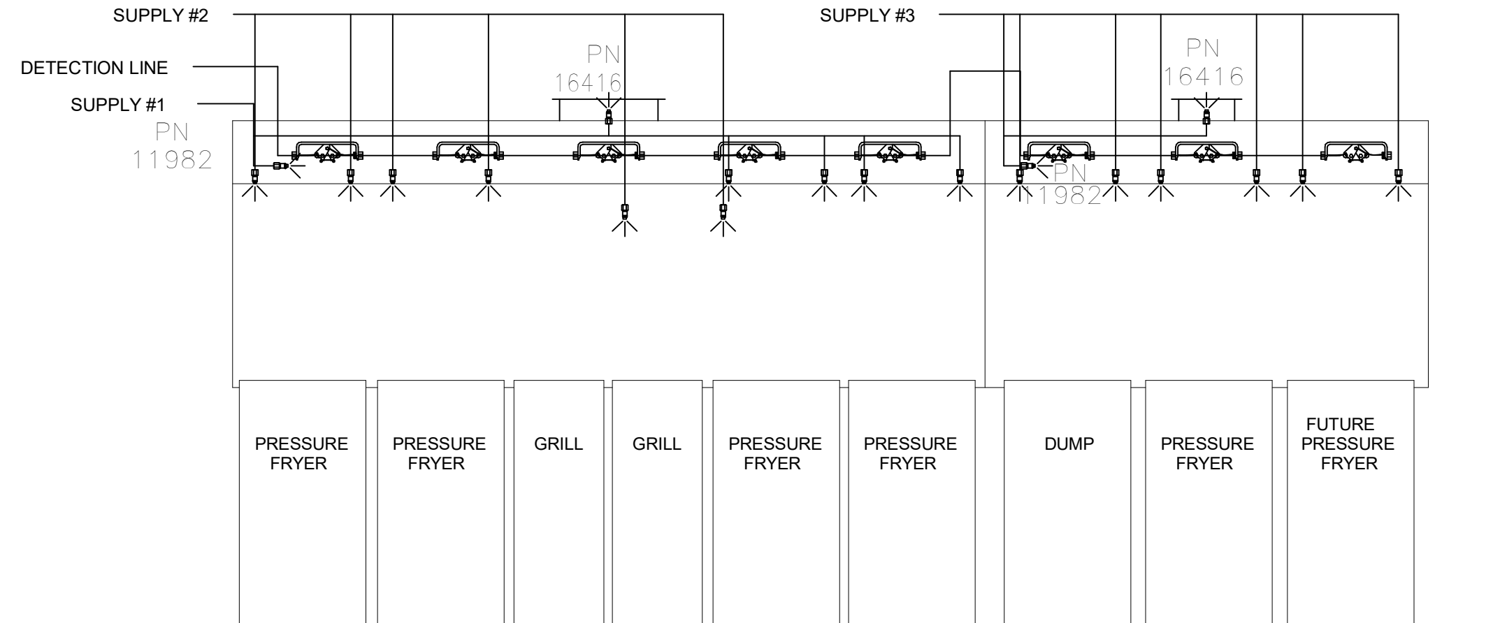
AMEREX FIRE SYSTEM LAYOUT
