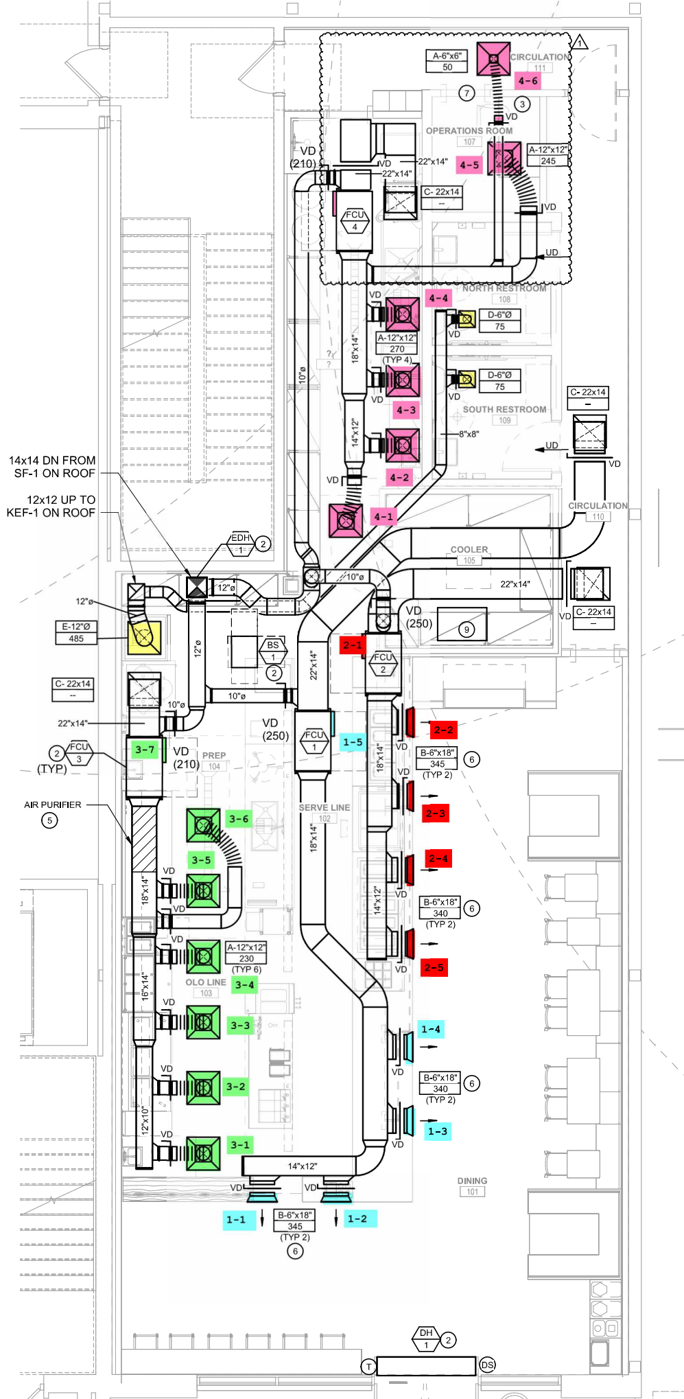
1 HVAC FIRST FLOOR DUCTWORK PLAN
