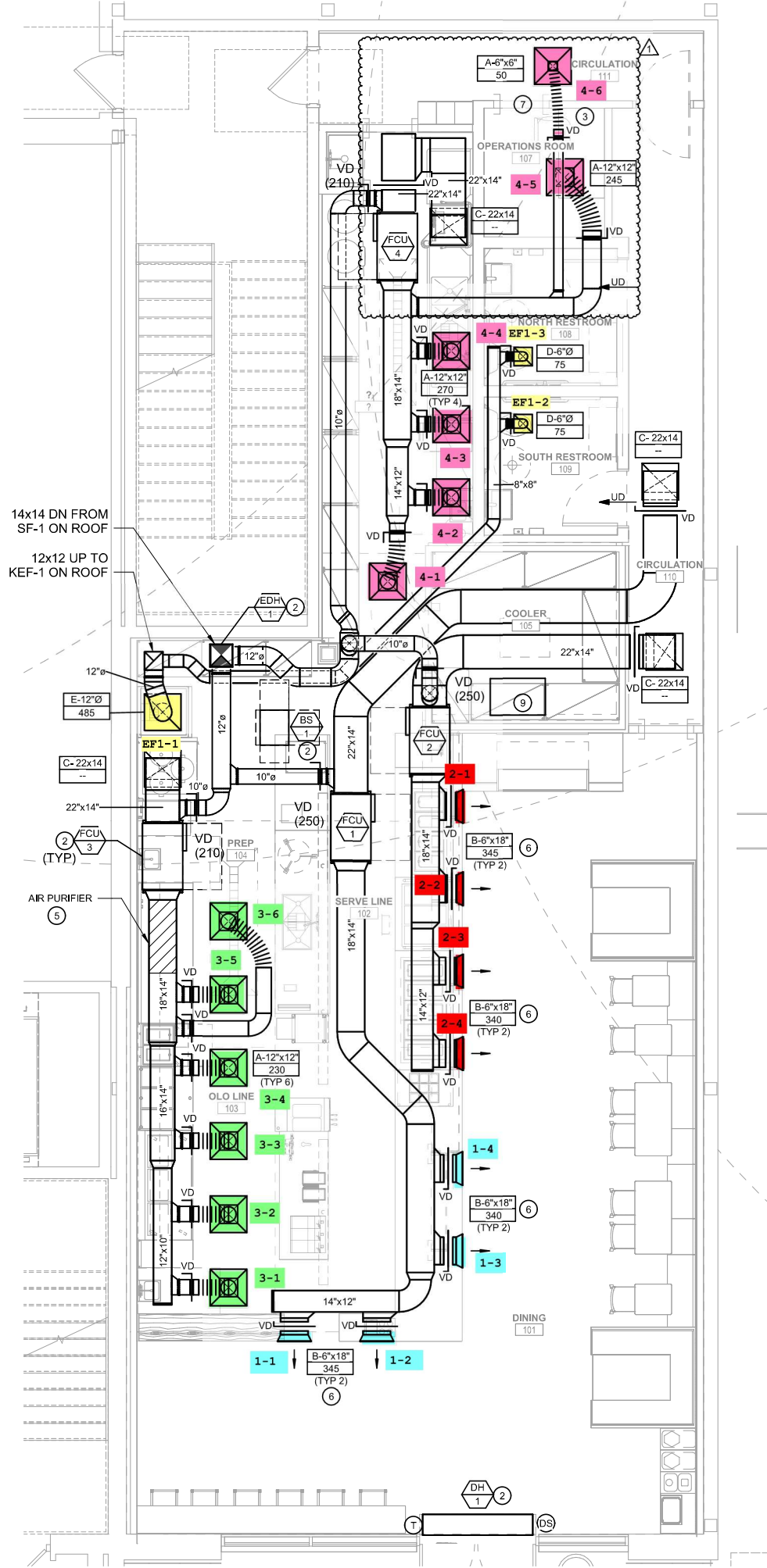
1 HVAC FIRST FLOOR DUCTWORK PLAN 1/4" = 1'-0"
